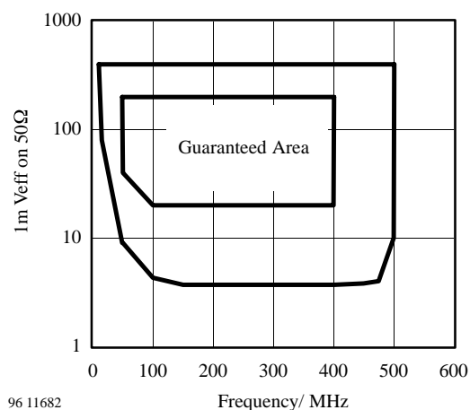
Figure 7. Input sensitivity of PLL2
