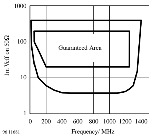
Figure 6. Input sensitivity of PLL1
