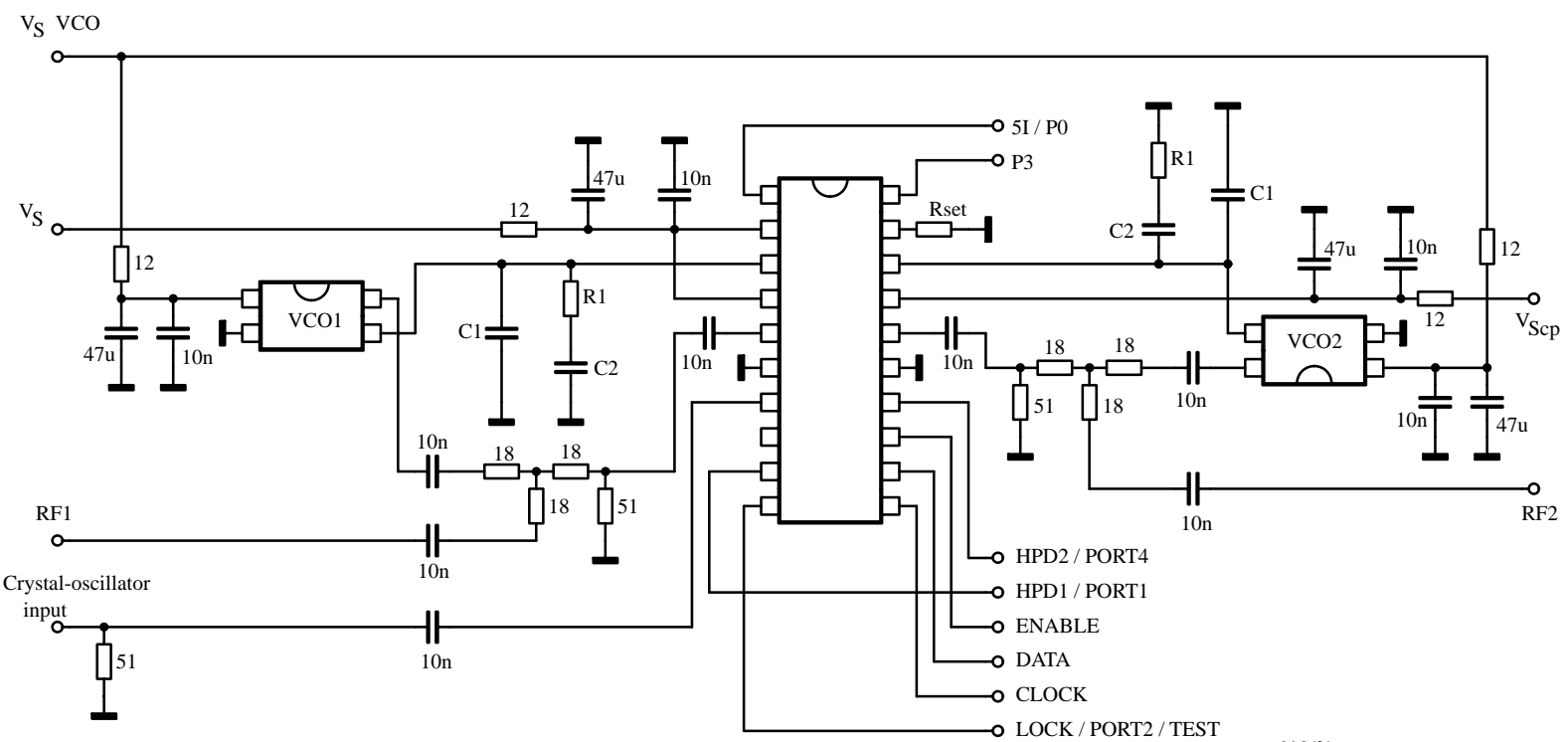
Figure 3. Application circuit
