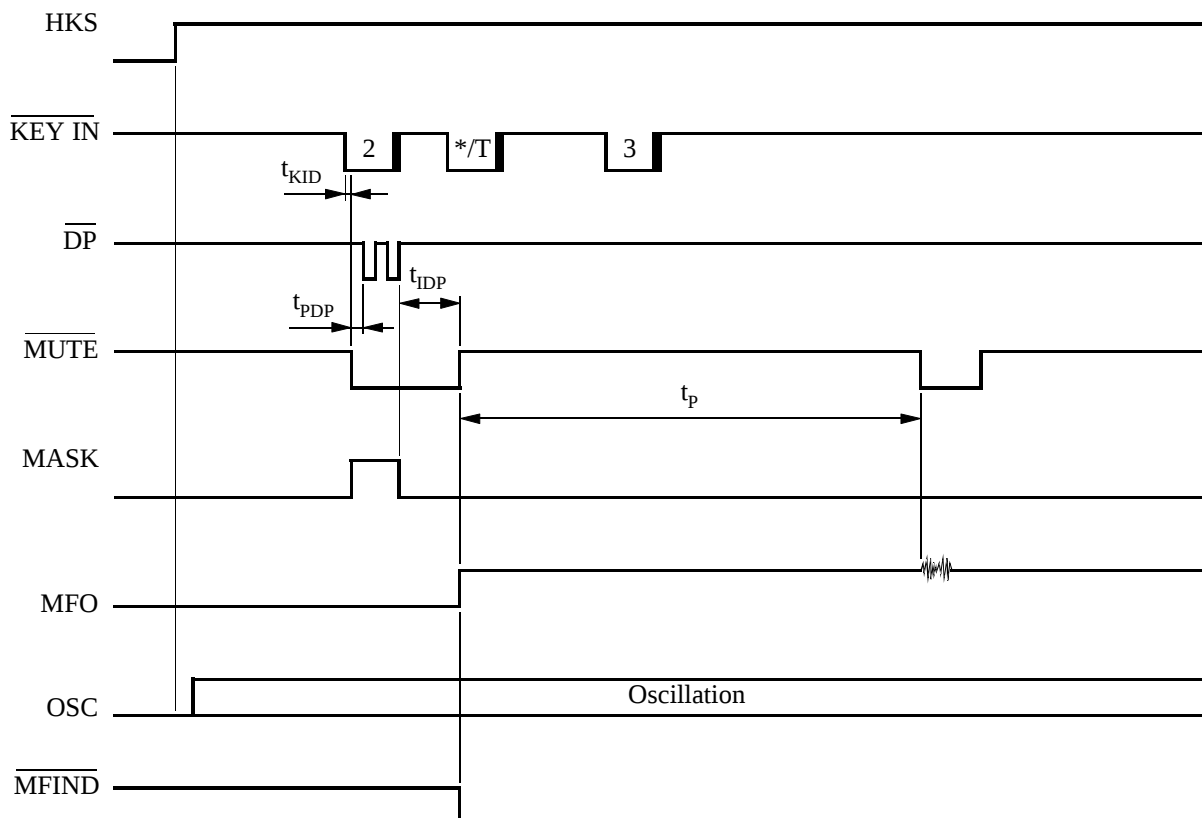
Figure 10. Pulse-to-tone operation
