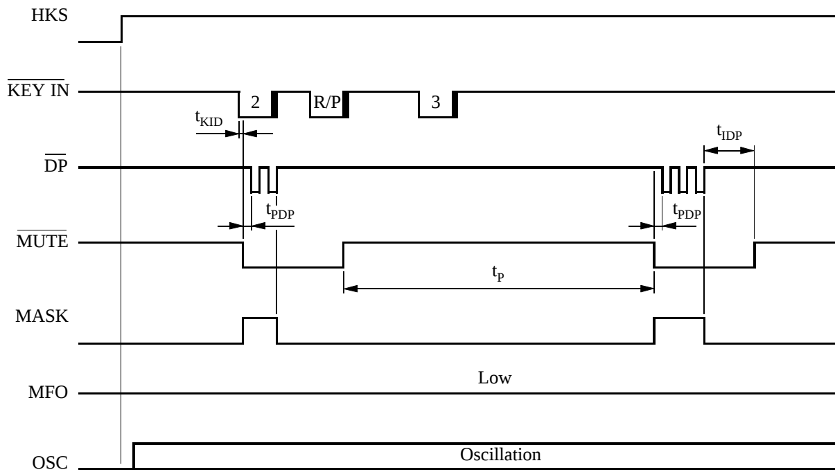
Figure 9. Pause function
