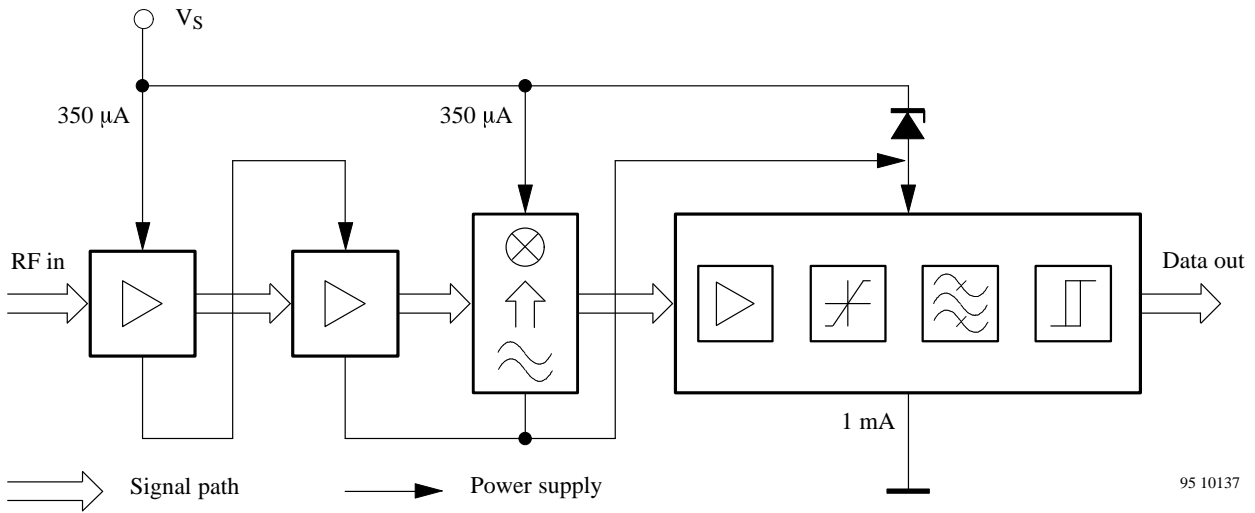
Figure 29. Principle diagram of a UHF remote-control receiver
