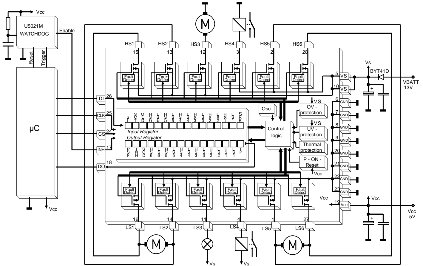
Figure 5. Application Circuit
