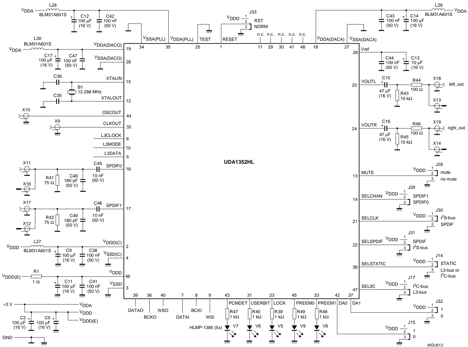
Fig.19 Application diagram.
