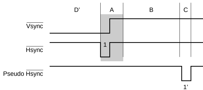
Figure 2-13. Synchronization Protection Circuit Operation (Mode 2)
