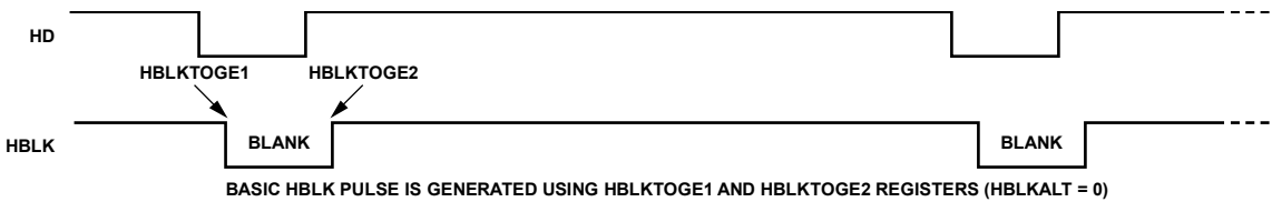
Figure 25. Typical Horizontal Blanking Pulse Placement (HBLKMODE = 0)
