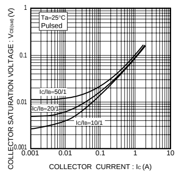
Fig.10 Collector-emitter saturation voltage vs. collector current
