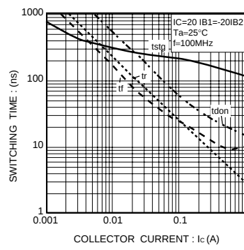
Fig.6 Switching time
