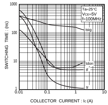
Fig.13 Switching time
