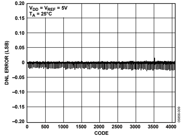
Figure 9. DNL AD5625, External Reference
