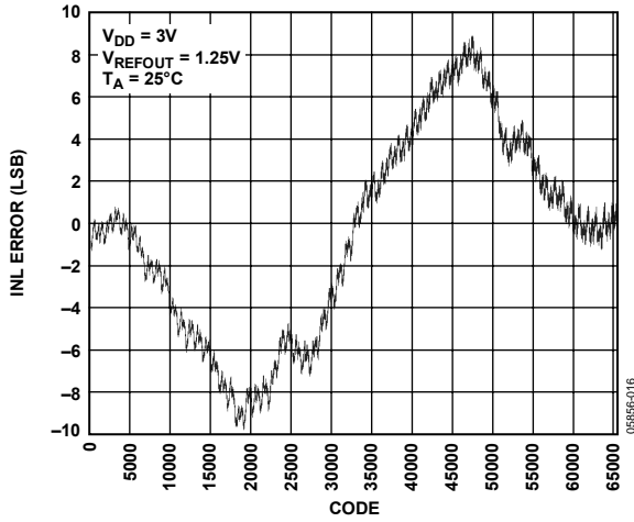
Figure 16. INL AD5665R, 1.25V Internal Reference
