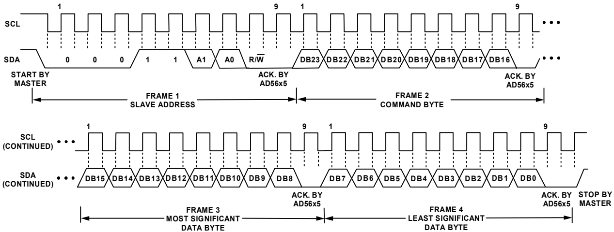
Figure 52. I 2 C Write Operation (10-Pin Package)
