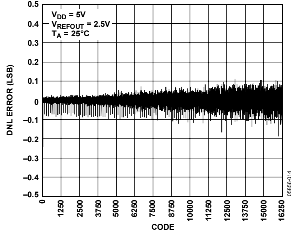
Figure 14. DNL AD5645R, 2.5V Internal Reference
