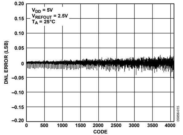
Figure 15. DNL AD5625R, 2.5V Internal Reference
