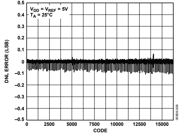
Figure 8. DNL AD5645, External Reference
