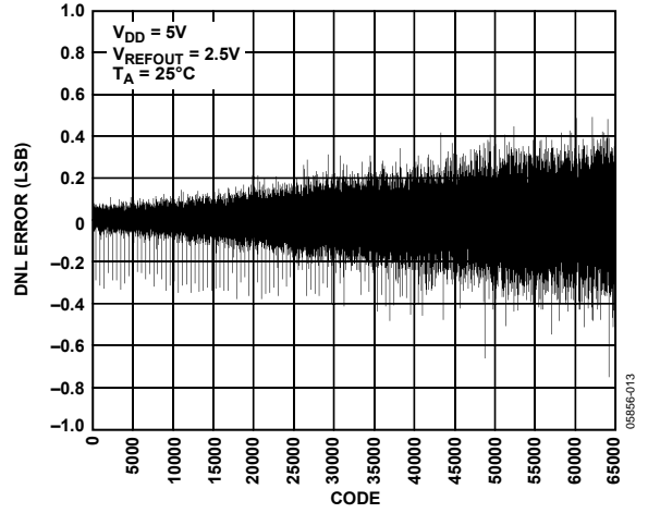
Figure 13. DNL AD5665R, 2.5V Internal Reference
