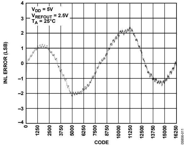
Figure 11. INL AD5645R, 2.5V Internal Reference
