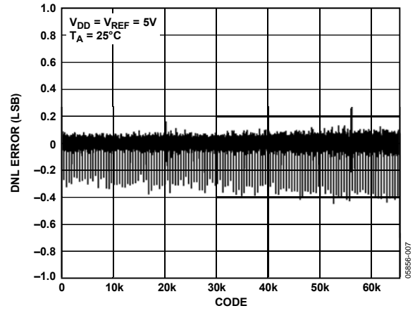
Figure 7. DNL AD5665, External Reference
