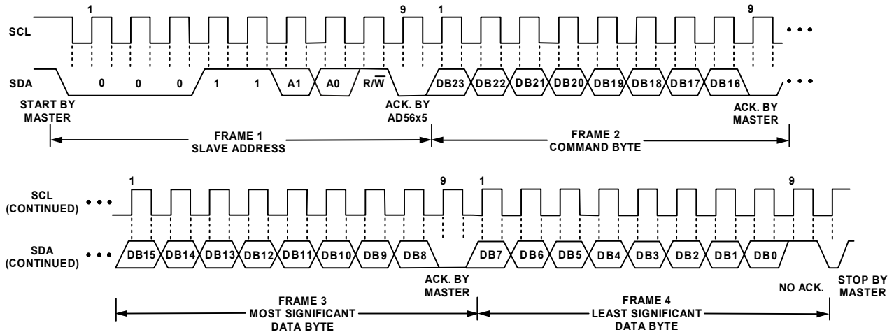
Figure 54. I 2 C Read Operation(10-Pin Package)
