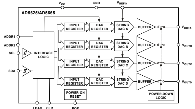
Figure 1. Functional Block Diagrams
