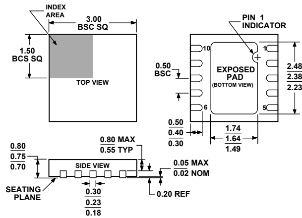
Figure 69. 10-Lead Lead Frame Chip Scale Package [LFCSP_WD] 3 mm x 3 mm Body, Very Very Thin, Dual Lead (CP-10-9) Dimensions shown in millimeters
