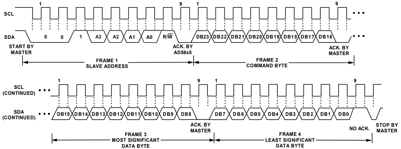
Figure 55. I 2 C Read Operation(14-Pin Package)
