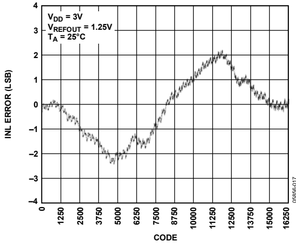
Figure 17. INL AD5645R, 1.25V Internal Reference
