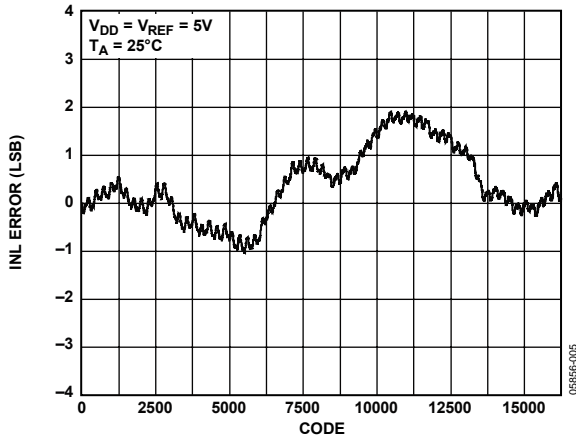
Figure 5. INL AD5645, External Reference
