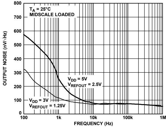
Figure 46. Noise Spectral Density, Internal Reference
