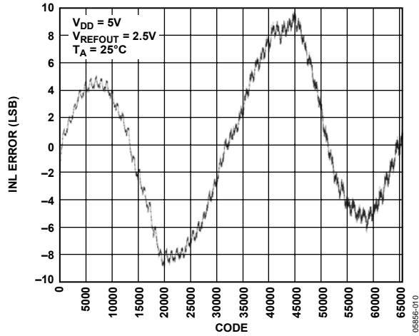
Figure 10. INL AD5665R, 2.5V Internal Reference
