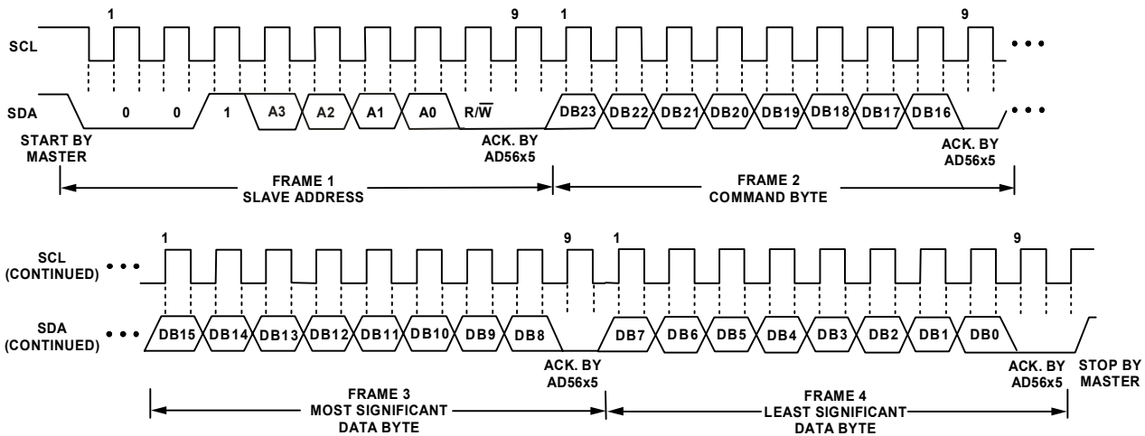
Figure 53. I 2 C Write Operation (14-Pin Package)
