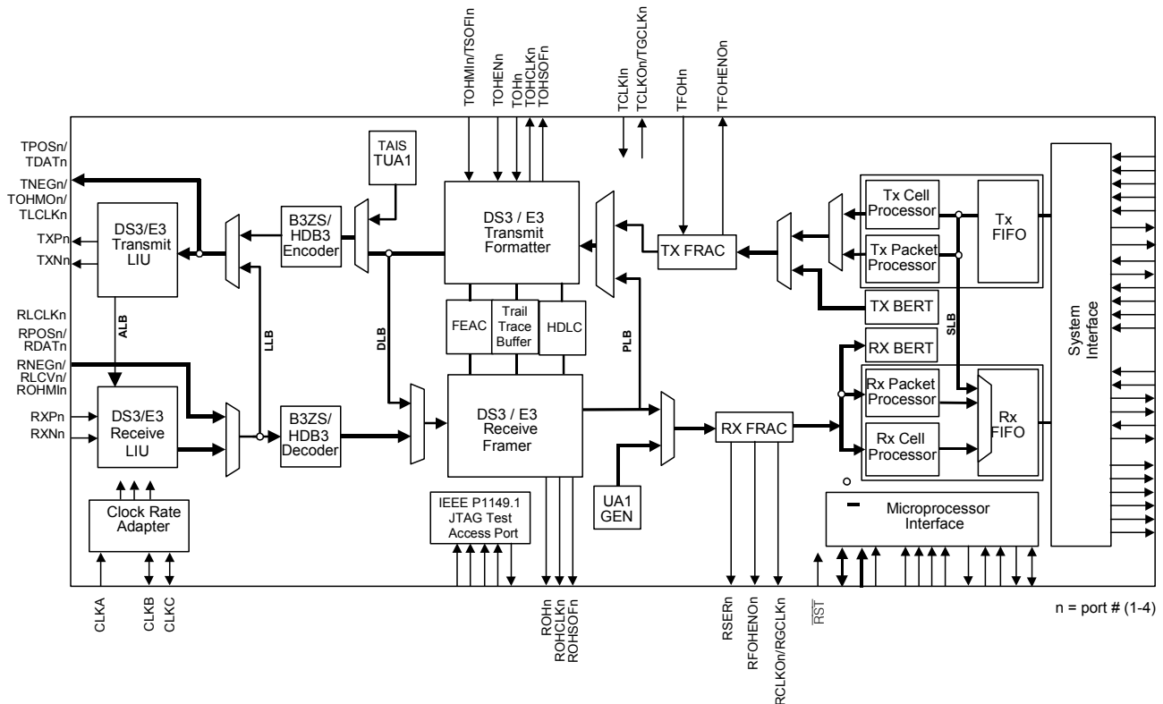
Figure 6-3. DS3/E3 Internal Fractional ATM/Packet Mode
