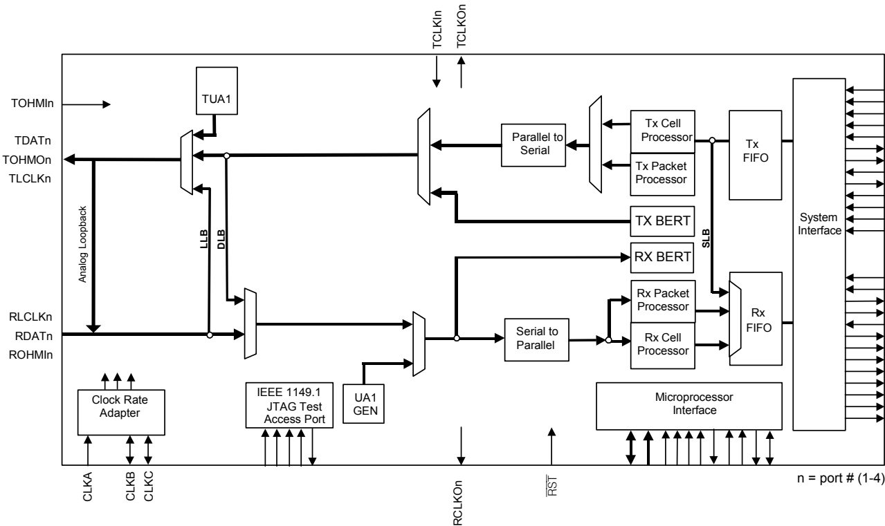
Figure 6-10. Clear-Channel Octet Aligned ATM/Packet—OHM Mode
