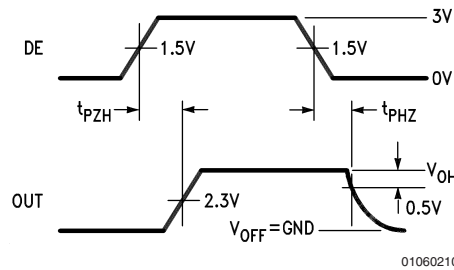
FIGURE 4. Driver Enable and Disable Timing (t PZH , t PHZ )
