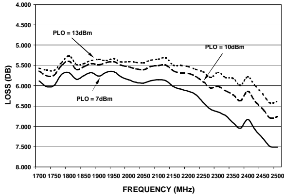
Conversion Loss
