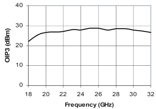
Figure 6. Output IP3
