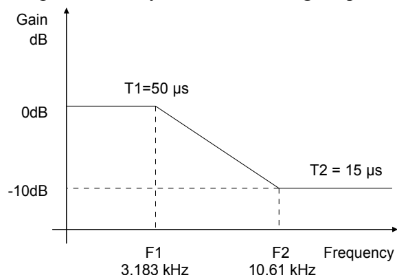
Figure 7. De-Emphasis Curve
