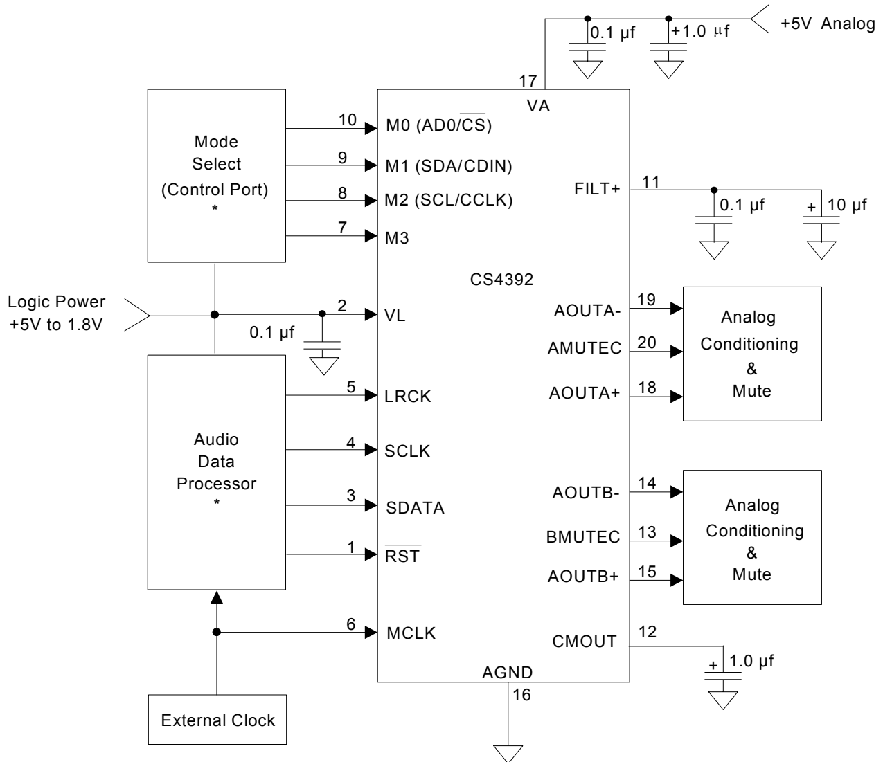
Figure 1. Typical Connection Diagram - PCM Mode * A high logic level for all digital inputs should not exceed VL.
