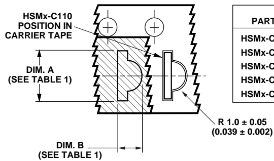
Figure 15. Tape dimensions.
