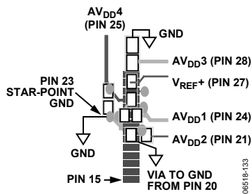
Figure 46. Supply Decoupling
