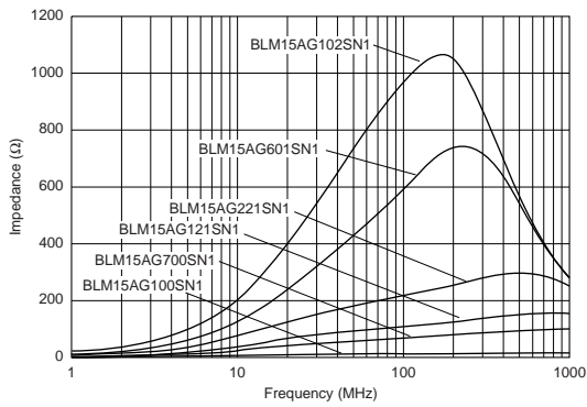
BLM15A Series
