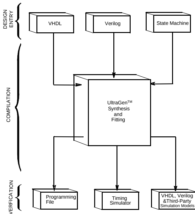
Figure 1. Warp VHDL Design Flow
