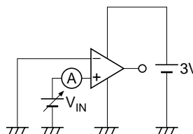
10. Input Bias Current, I_{IB}
