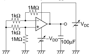
8. Input Offset Voltage vs. V_{DD}
