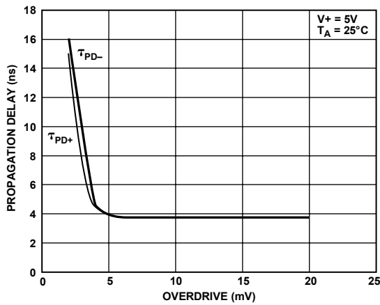
Figure 8. Propagation Delay vs. Overdrive
