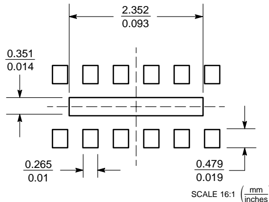
SOLDERING FOOTPRINT*
