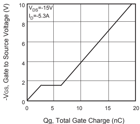
Figure 15. Gate Charge
