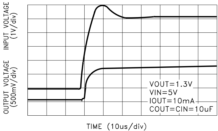
TURN-ON TIME
