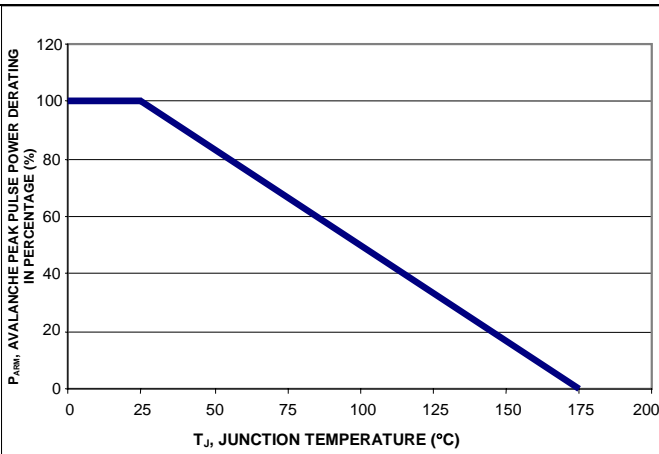
Figure 4: Pulse Derating Curve, Per Element
