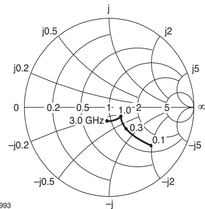
Figure 8. Output Reflection Coefficient
