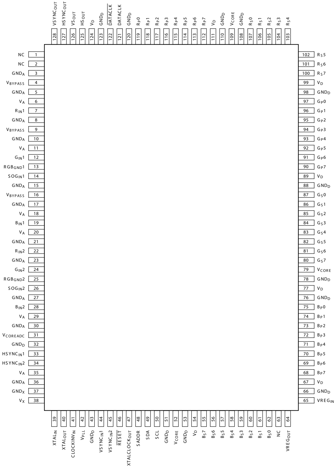
X98027 (128-PIN MQFP) TOP VIEW
