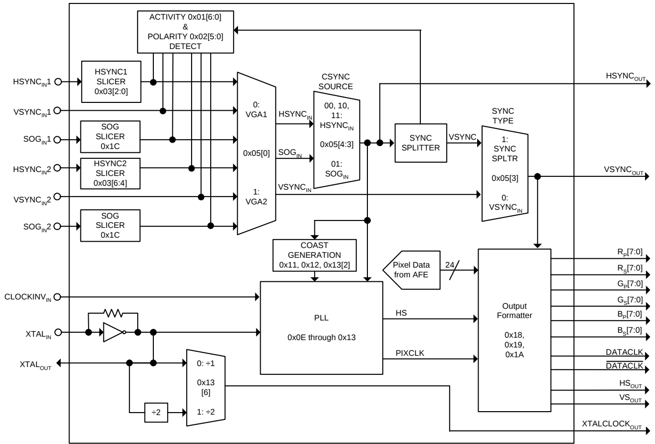
FIGURE 8. SYNC FLOW
