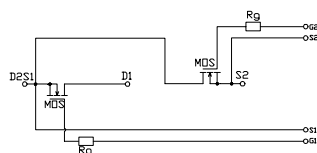
Circuit
