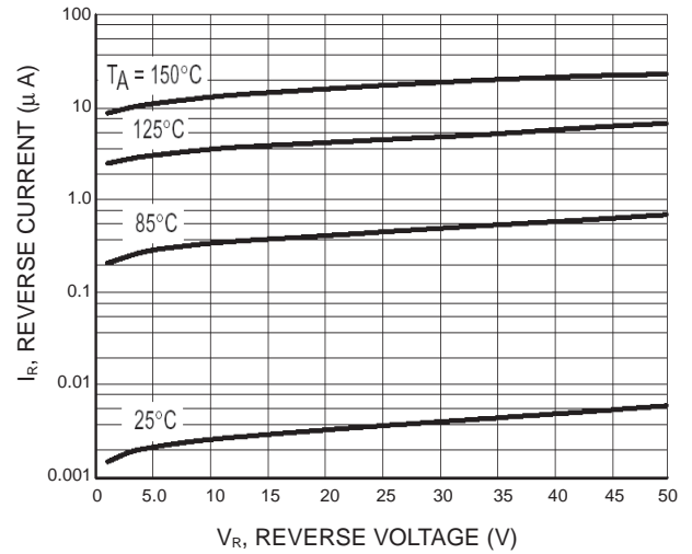
Figure 2. Reverse Current Versus Reverse Voltage
