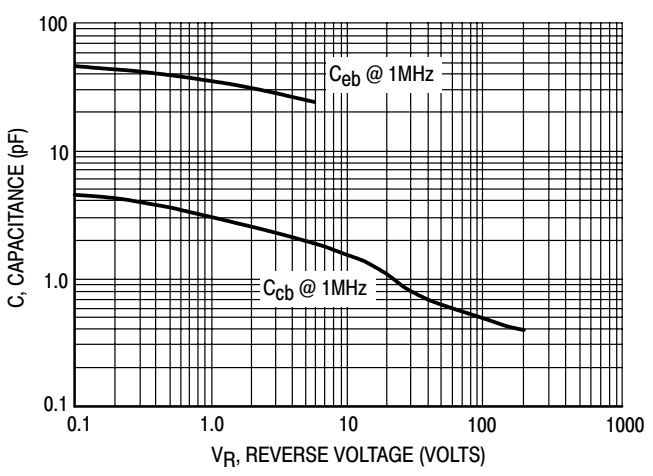
Figure 2. Capacitance
