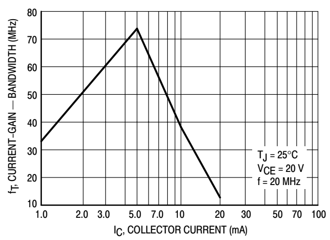
Figure 3. Current-Gain - Bandwidth
