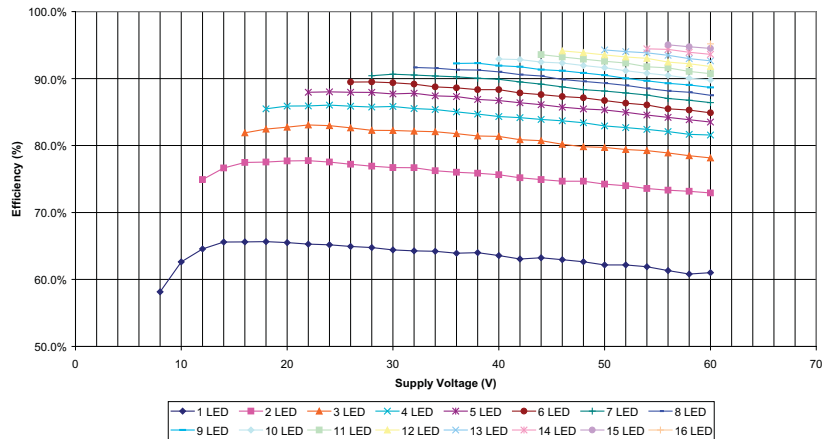
ZXLD1362 Efficiency L=100\mu\text{H}
