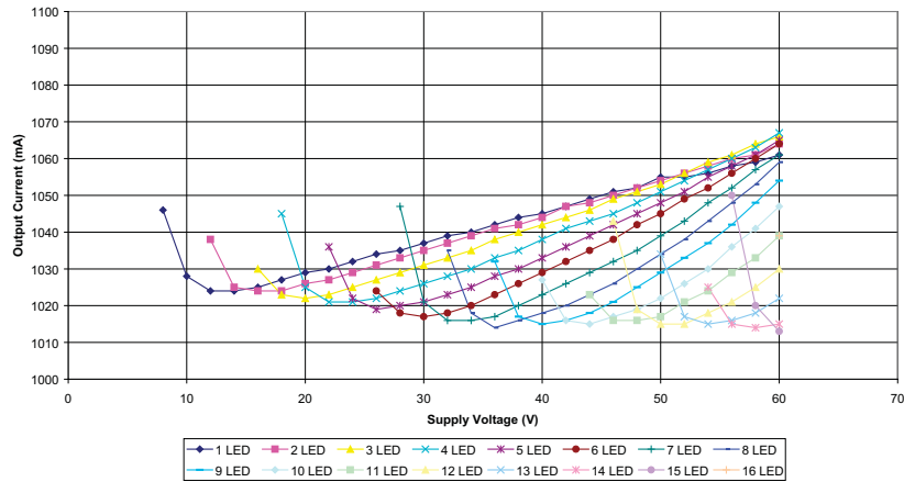
ZXLD1362 Output Current L=100\mu\text{H}
