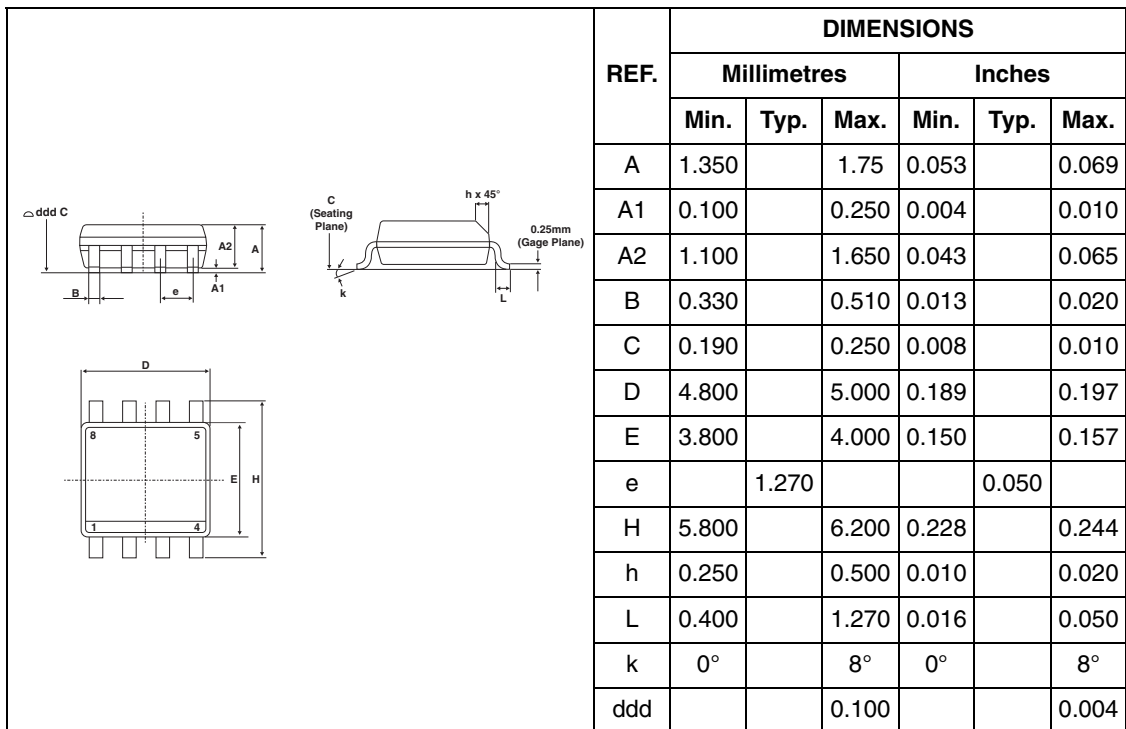
Figure 18. SO-8 Footprint
