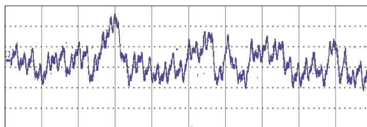
Typical Peak-to-Peak Noise of ACS706ELC-05C at T_A=25^\circ\text{C}
