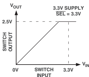
Figure 6. 3.3 V to 2.5 V Voltage Translation, \overline{SEL} = V_{CC}
