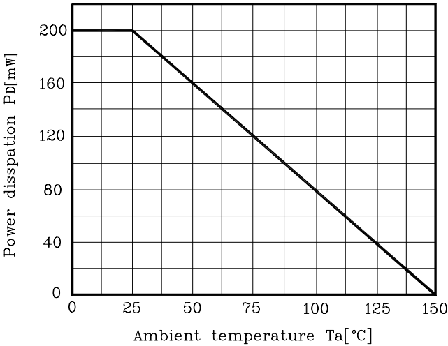
Fig. 1 P_D - T_a
