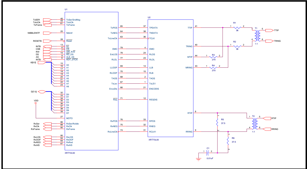
FIGURE 118. INTERFACING THE XRT72L52 FRAMER IC TO THE XRT73L00 DS3/E3/STS-1 LIU
