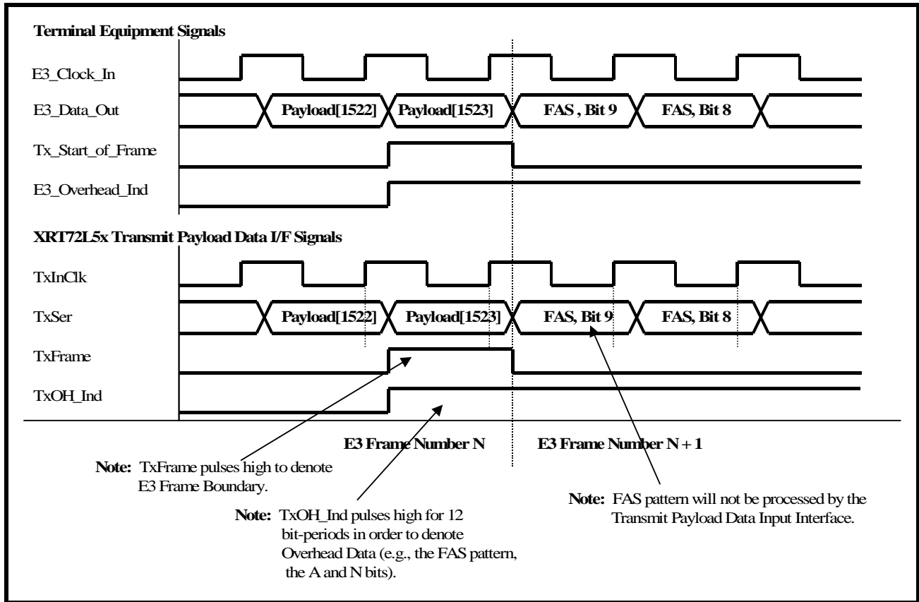
FIGURE 93. BEHAVIOR OF THE TERMINAL INTERFACE SIGNALS BETWEEN THE XRT72L52 AND THE TERMINAL EQUIPMENT (E3 MODE 3 OPERATION)
