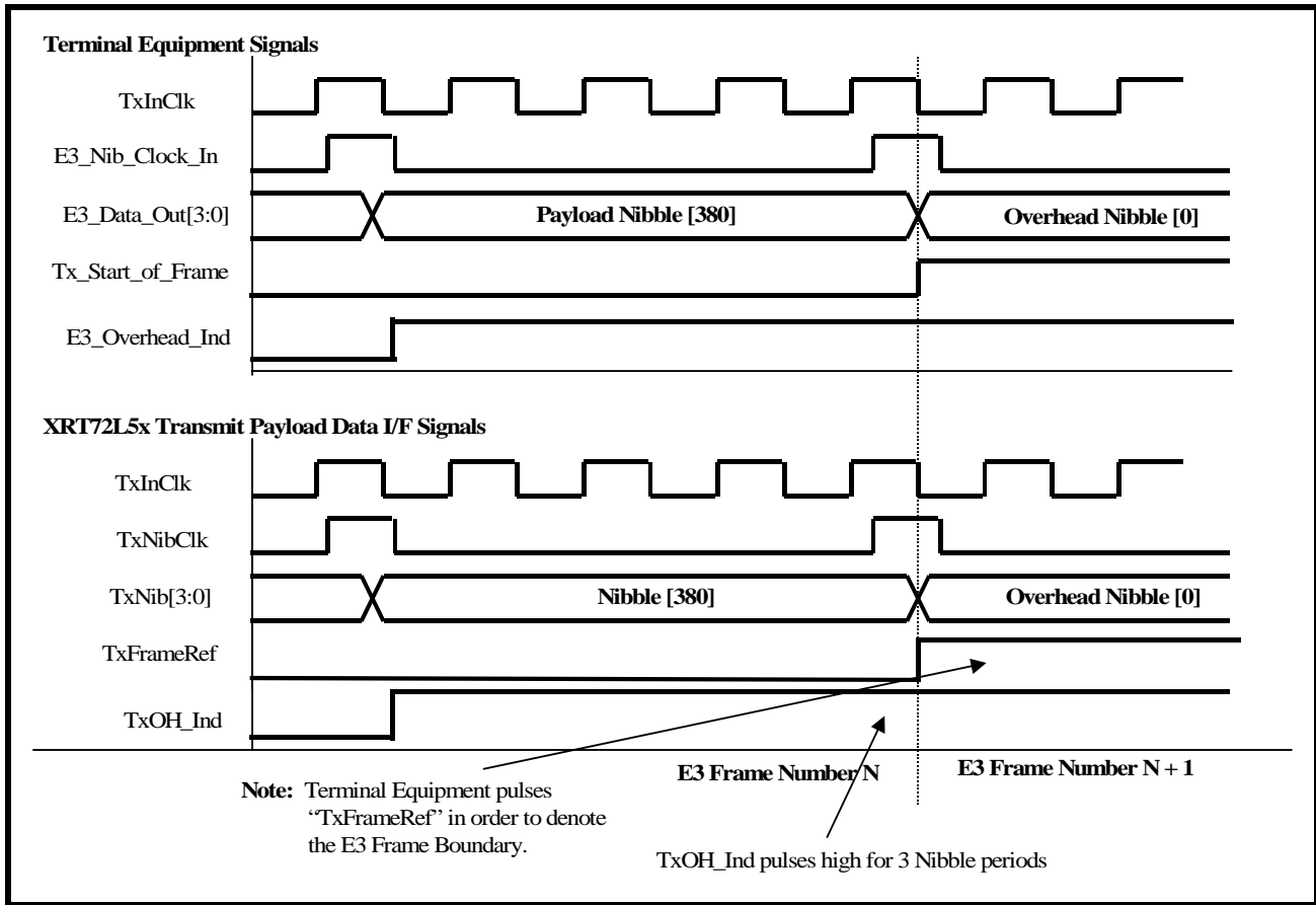
FIGURE 97. BEHAVIOR OF THE TERMINAL INTERFACE SIGNALS BETWEEN THE XRT72L52 AND THE TERMINAL EQUIPMENT (E3, MODE 5 OPERATION)
