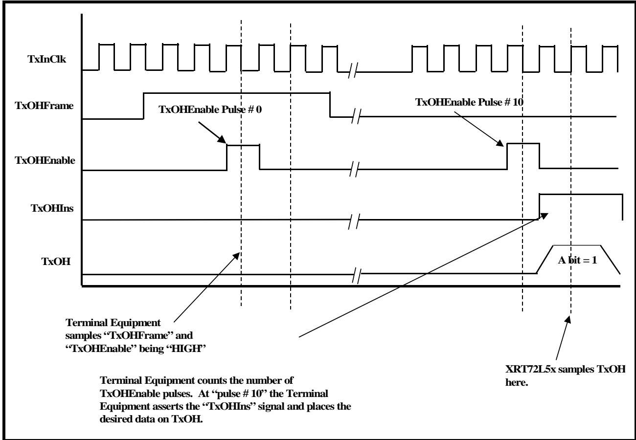
FIGURE 104. BEHAVIOR OF TRANSMIT OVERHEAD DATA INPUT INTERFACE SIGNALS BETWEEN THE XRT72L52 AND THE TERMINAL EQUIPMENT (FOR METHOD 2)
