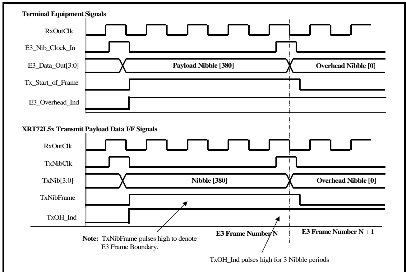
FIGURE 95. BEHAVIOR OF THE TERMINAL INTERFACE SIGNALS BETWEEN THE XRT72L52 AND THE TERMINAL EQUIPMENT (MODE 4 OPERATION)
