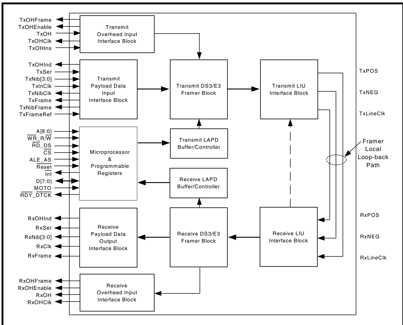
FIGURE 200. THE FRAMER LOCAL LOOP-BACK PATH WITHIN THE XRT72L52 DS3/E3 FRAMER IC
