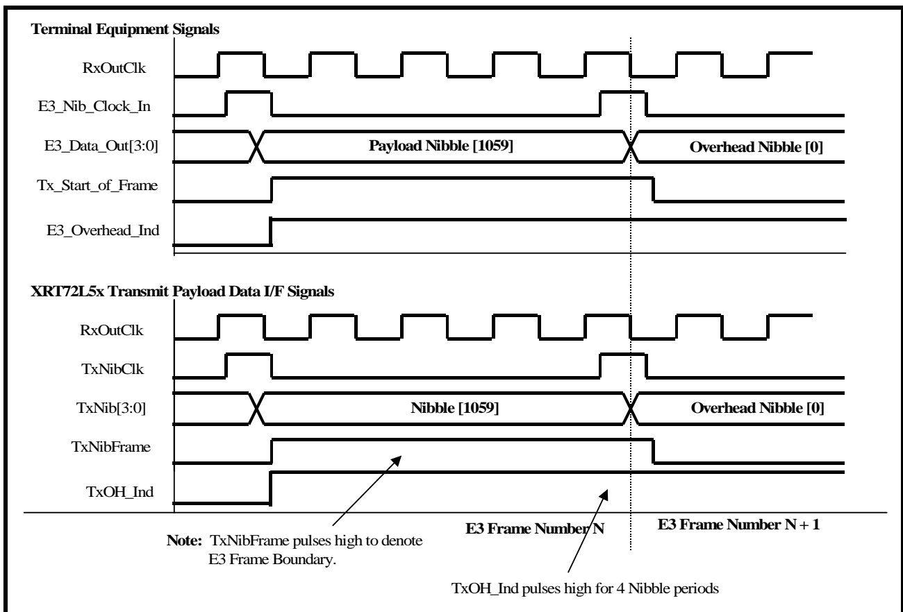
FIGURE 152. BEHAVIOR OF THE TERMINAL INTERFACE SIGNALS BETWEEN THE XRT72L52 AND THE TERMINAL EQUIPMENT (MODE 4 OPERATION)
