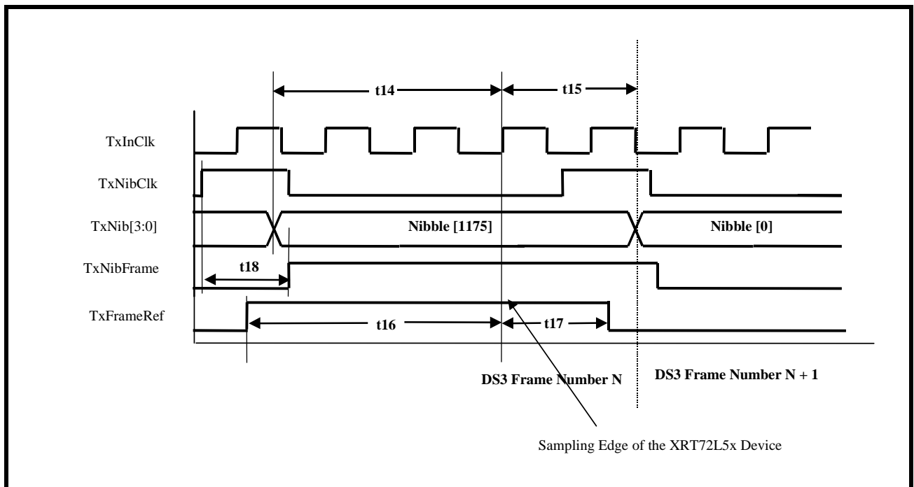
FIGURE 6. TIMING DIAGRAM FOR THE TRANSMIT PAYLOAD DATA INPUT INTERFACE, WHEN THE XRT72L52 IS OPERATING IN THE DS3/NIBBLE AND LOCAL-TIMING MODES
