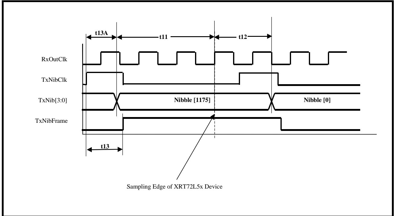
FIGURE 5. TIMING DIAGRAM FOR THE TRANSMIT PAYLOAD DATA INPUT INTERFACE, WHEN THE XRT72L52 IS OPERATING IN BOTH THE DS3/NIBBLE AND LOOPED-TIMING MODES
