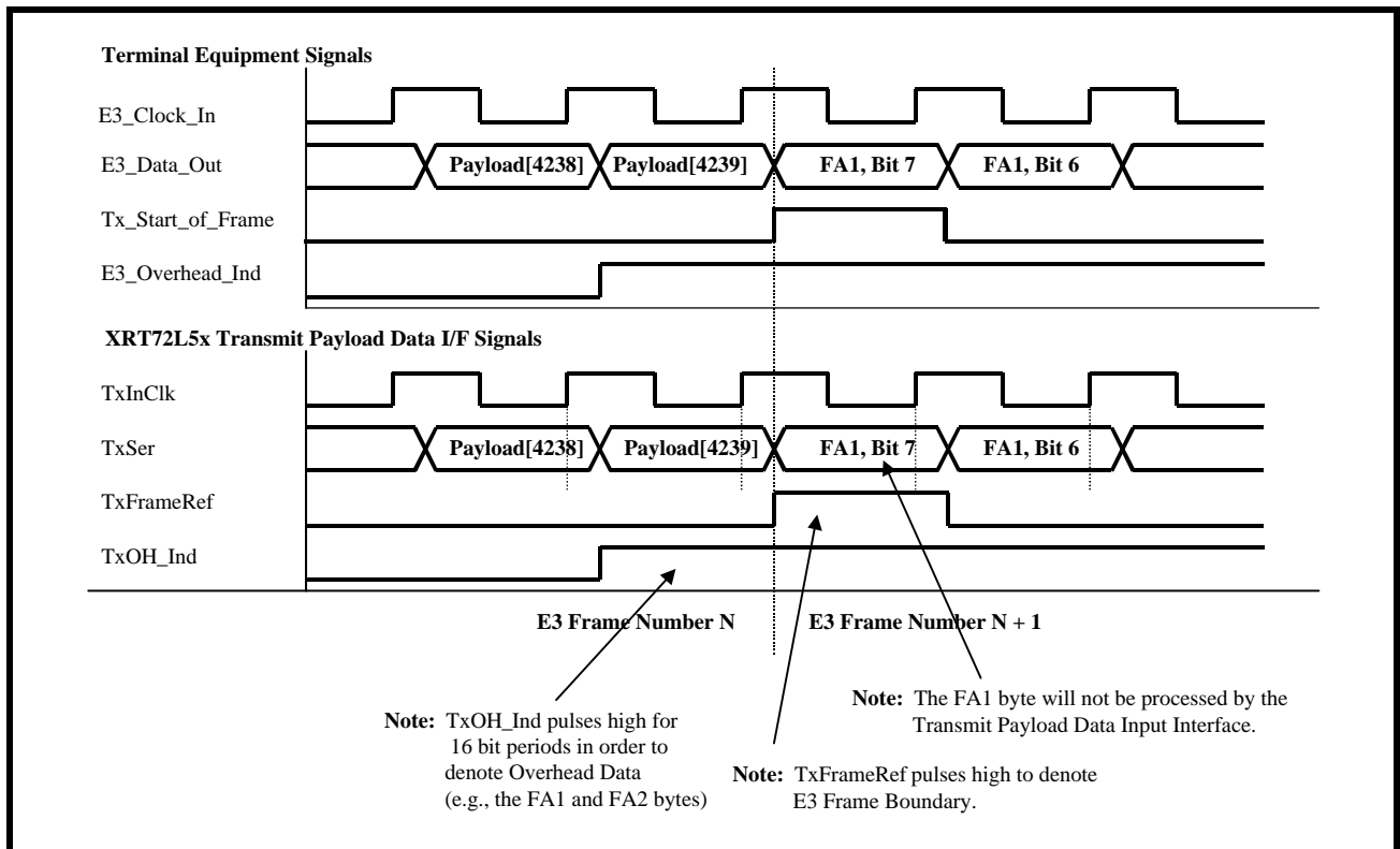
FIGURE 148. BEHAVIOR OF THE TERMINAL INTERFACE SIGNALS BETWEEN THE XRT72L52 AND THE TERMINAL EQUIPMENT (MODE 2 OPERATION)
