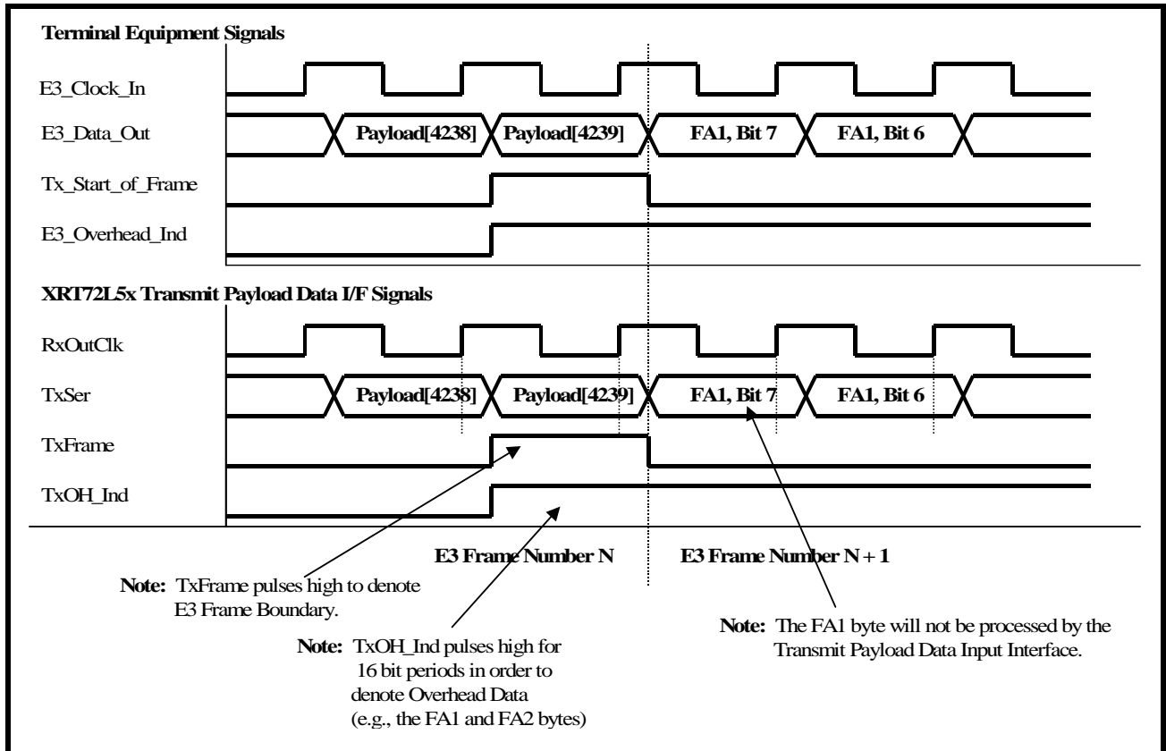
FIGURE 146. BEHAVIOR OF THE TERMINAL INTERFACE SIGNALS BETWEEN THE TRANSMIT PAYLOAD DATA INPUT INTERFACE BLOCK OF THE XRT72L52 AND THE TERMINAL EQUIPMENT (FOR MODE 1 OPERATION)
