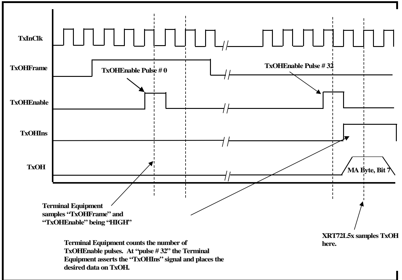
FIGURE 161. BEHAVIOR OF TRANSMIT OVERHEAD DATA INPUT INTERFACE SIGNALS BETWEEN THE XRT72L52 AND THE TERMINAL EQUIPMENT (FOR METHOD 2)
