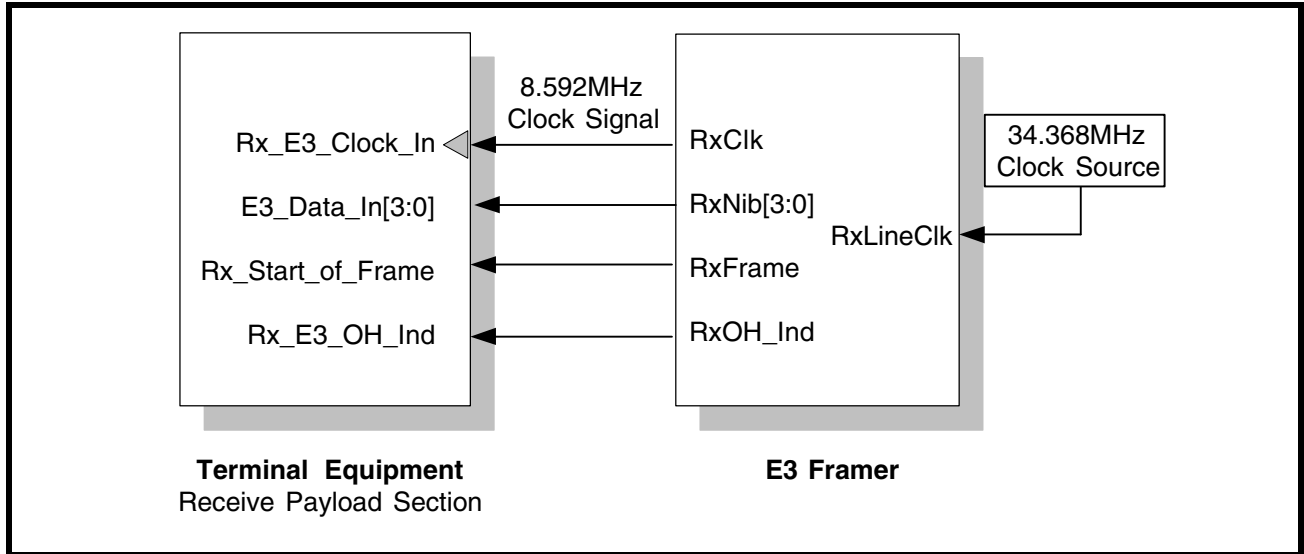
FIGURE 140. THE XRT72L52 DS3/E3 FRAMER IC BEING INTERFACED TO THE RECEIVE SECTION OF THE TERMINAL EQUIPMENT (NIBBLE-PARALLEL MODE OPERATION)
