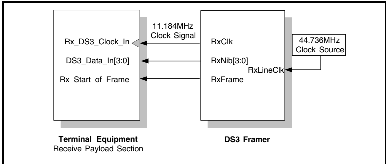
FIGURE 83. THE XRT72L52 DS3/E3 FRAMER IC BEING INTERFACED TO THE RECEIVE SECTION OF THE TERMINAL EQUIPMENT (NIBBLE-PARALLEL MODE OPERATION)
