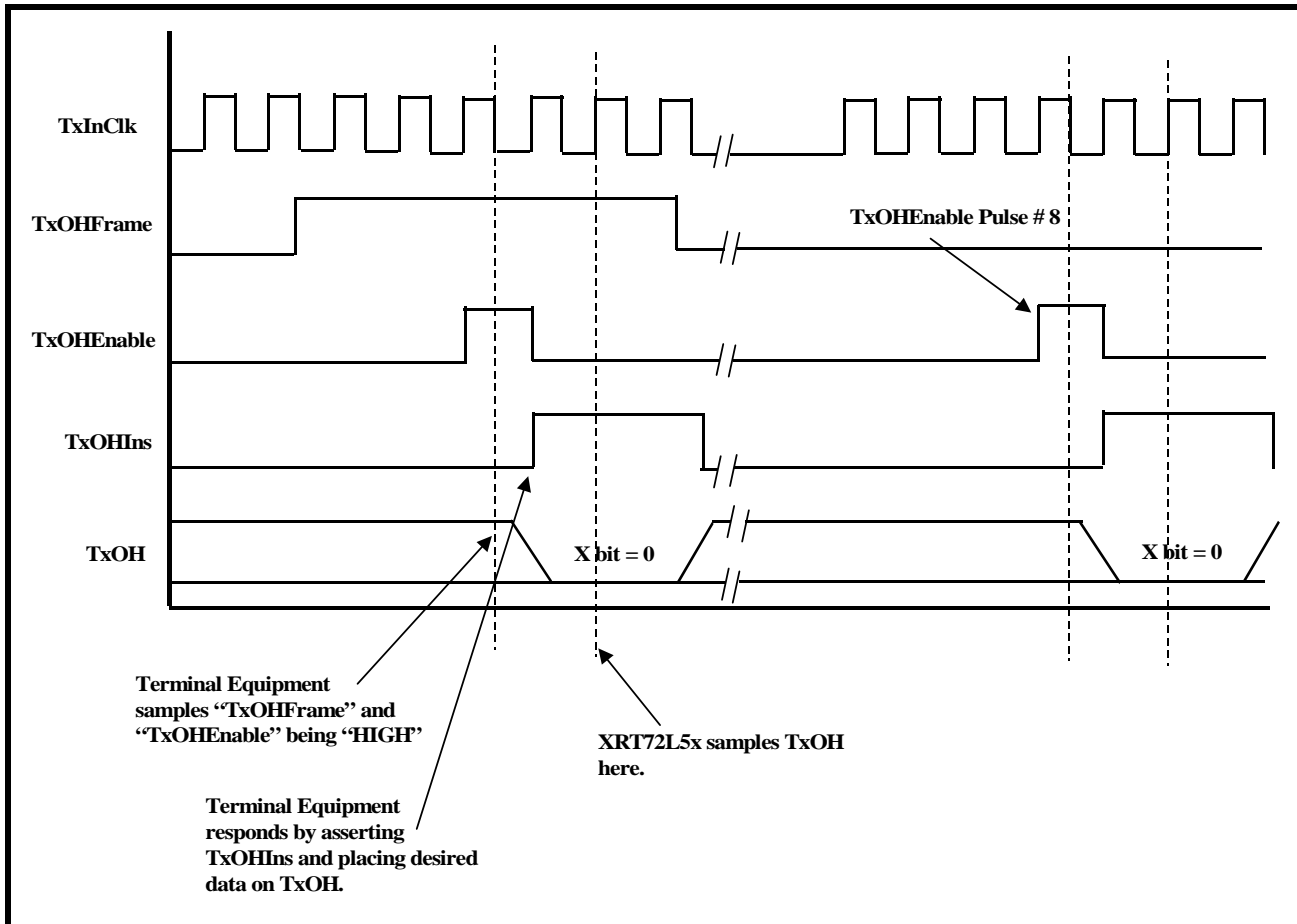
FIGURE 48. BEHAVIOR OF TRANSMIT OVERHEAD DATA INPUT INTERFACE SIGNALS BETWEEN THE XRT72L52 AND THE TERMINAL EQUIPMENT (FOR METHOD 2)
