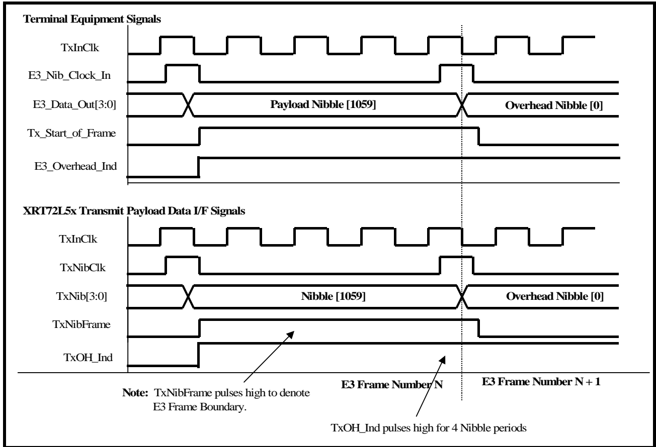
FIGURE 156. BEHAVIOR OF THE TERMINAL INTERFACE SIGNALS BETWEEN THE XRT72L52 AND THE TERMINAL EQUIPMENT (E3 MODE 6 OPERATION)
