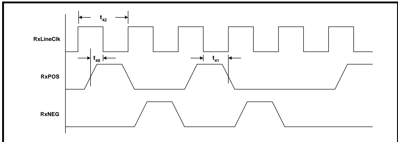
FIGURE 67. WAVEFORM/TIMING RELATIONSHIP BETWEEN RxLINECLK, RxPOS AND RxNEG - WHEN RxPOS AND RxNEG ARE TO BE SAMPLED ON THE FALLING EDGE OF RxLINECLK
