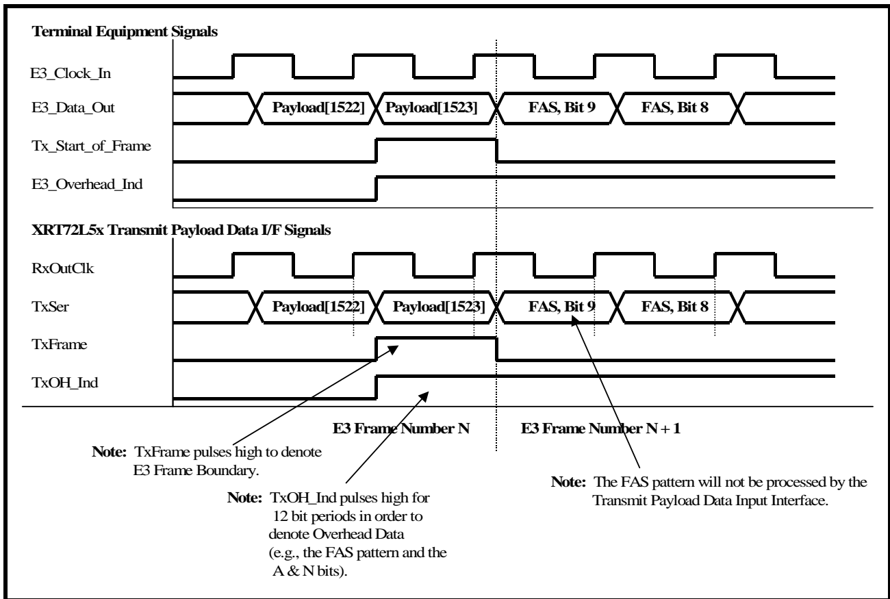
FIGURE 89. BEHAVIOR OF THE TERMINAL INTERFACE SIGNALS BETWEEN THE XRT72L52 TRANSMIT PAYLOAD DATA INPUT INTERFACE BLOCK AND THE TERMINAL EQUIPMENT (FOR MODE 1 OPERATION)
