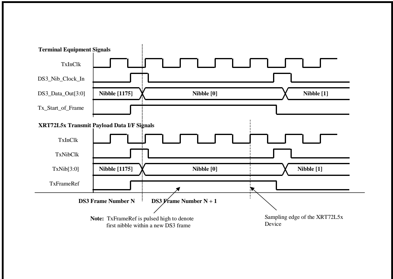
FIGURE 41. BEHAVIOR OF THE TERMINAL INTERFACE SIGNALS BETWEEN THE XRT72L52 AND THE TERMINAL EQUIPMENT (DS3 MODE 5 OPERATION)
