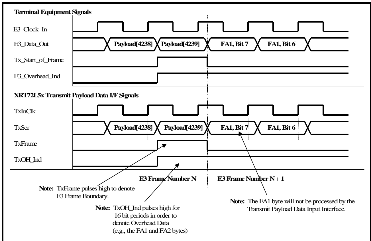
FIGURE 150. BEHAVIOR OF THE TERMINAL INTERFACE SIGNALS BETWEEN THE XRT72L52 AND THE TERMINAL EQUIPMENT (E3 MODE 3 OPERATION)
