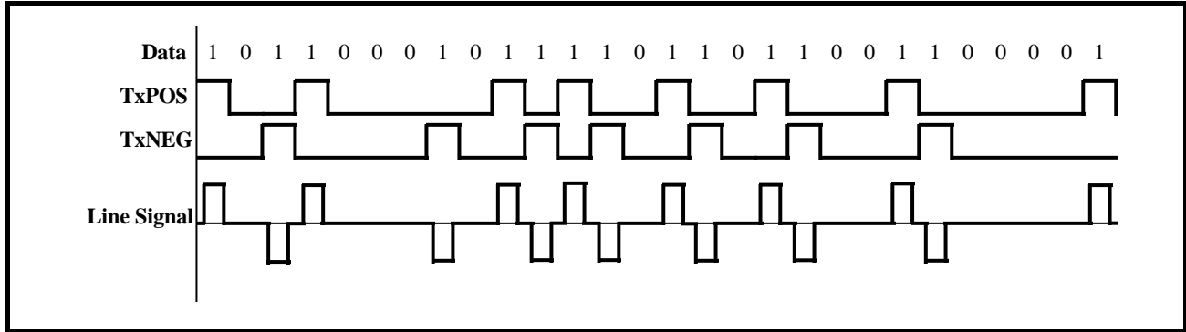
FIGURE 111. ILLUSTRATION OF AMI LINE CODE
