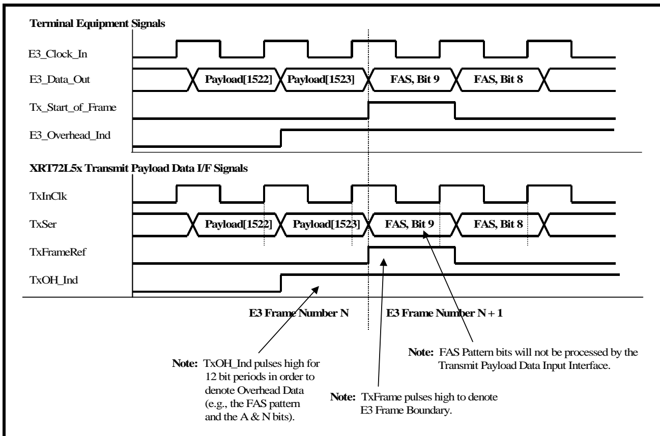
FIGURE 91. BEHAVIOR OF THE TERMINAL INTERFACE SIGNALS BETWEEN THE XRT72L52 AND THE TERMINAL EQUIPMENT (MODE 2 OPERATION)
