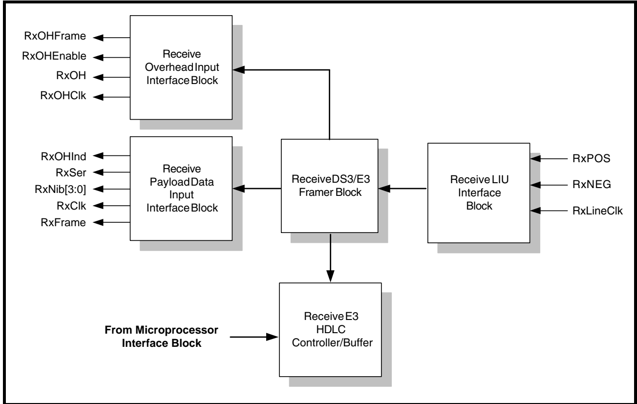
FIGURE 115. THE XRT72L52 RECEIVE SECTION CONFIGURED TO OPERATE IN THE E3 MODE
