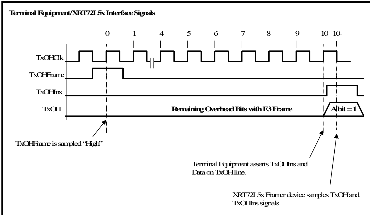
FIGURE 102. ILLUSTRATION OF THE SIGNAL THAT MUST OCCUR BETWEEN THE TERMINAL EQUIPMENT AND THE XRT72L52 IN ORDER TO CONFIGURE THE XRT72L52 TO TRANSMIT A YELLOW ALARM TO THE REMOTE TERMINAL EQUIPMENT
