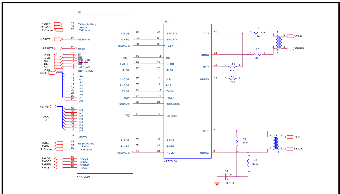
FIGURE 27. XRT72L52 DS3/E3 FRAMER INTERFACED TO THE XRT73L02A DS3/E3/STS-1 LIU
