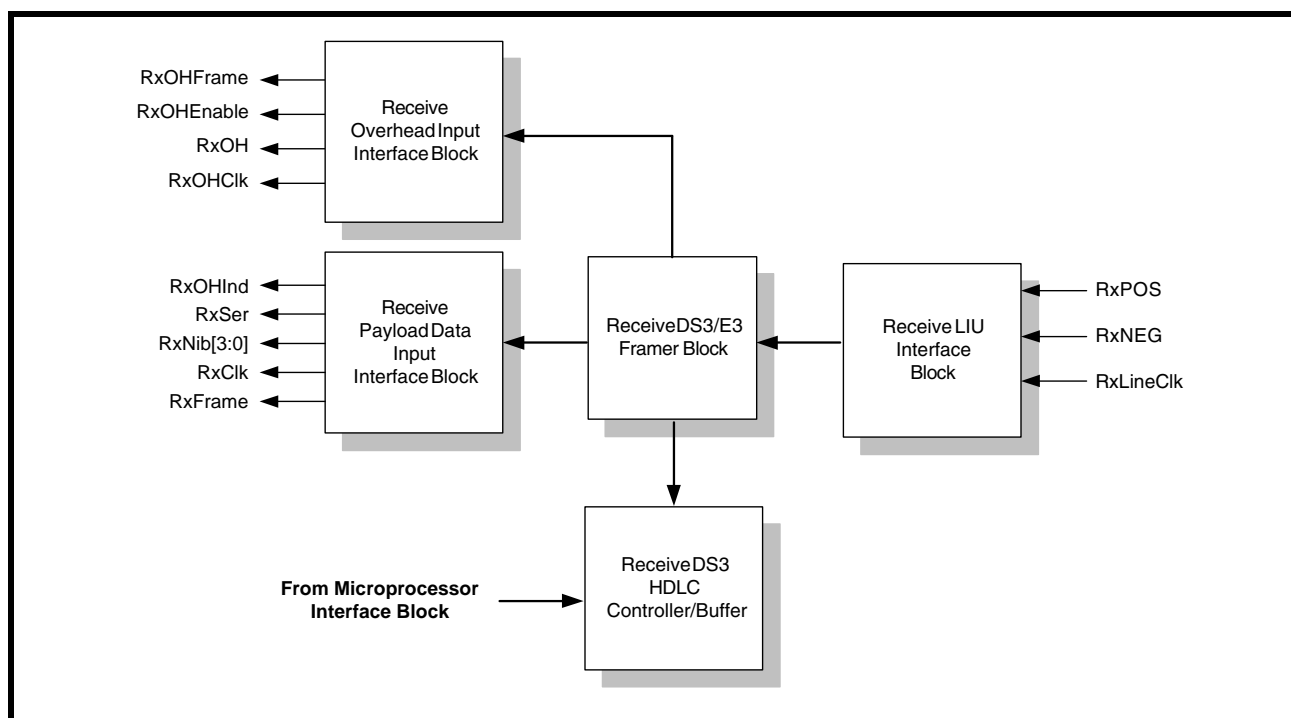
FIGURE 60. THE XRT72L52 RECEIVE SECTION CONFIGURED TO OPERATE IN THE DS3 MODE
