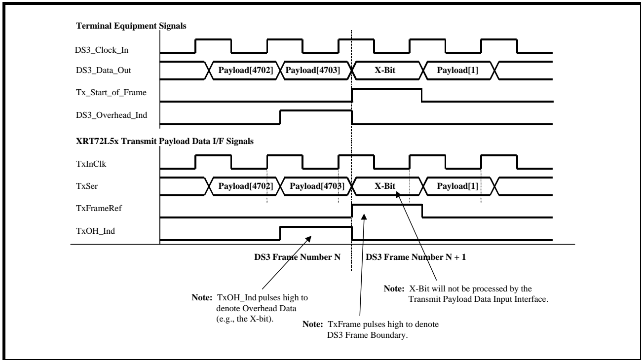
FIGURE 35. BEHAVIOR OF THE TERMINAL INTERFACE SIGNALS BETWEEN THE XRT72L52 AND THE TERMINAL EQUIPMENT (MODE 2 OPERATION)
