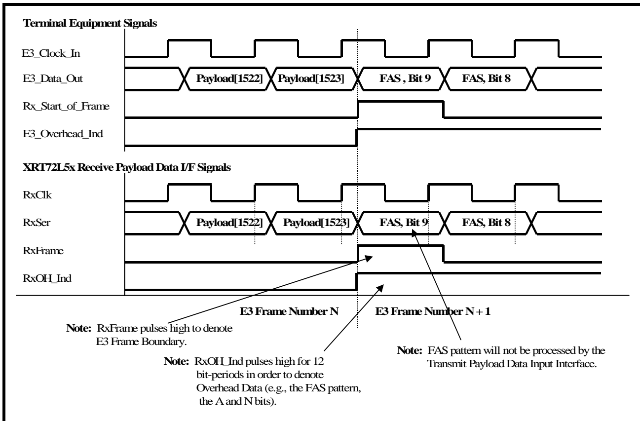
FIGURE 139. AN ILLUSTRATION OF THE BEHAVIOR OF THE SIGNALS BETWEEN THE RECEIVE PAYLOAD DATA OUTPUT INTERFACE BLOCK OF THE XRT72L52 AND THE TERMINAL EQUIPMENT
