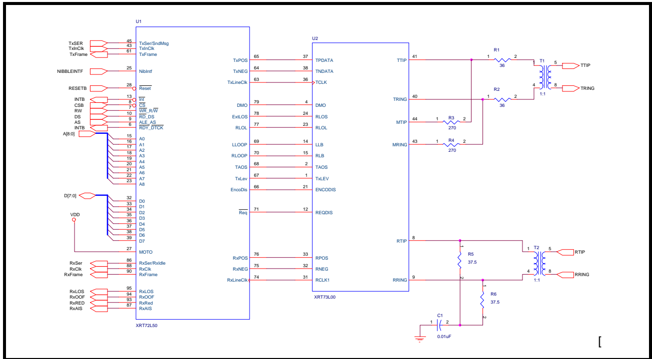
FIGURE 176. INTERFACING THE XRT72L52 FRAMER IC TO THE XRT73L00 DS3/E3/STS-1 LIU
