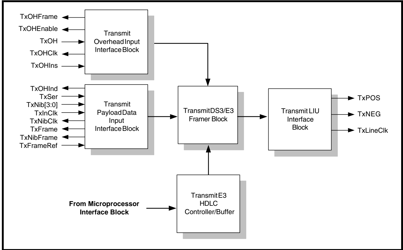
FIGURE 86. THE XRT72L52 TRANSMIT SECTION CONFIGURED TO OPERATE IN THE E3 MODE
