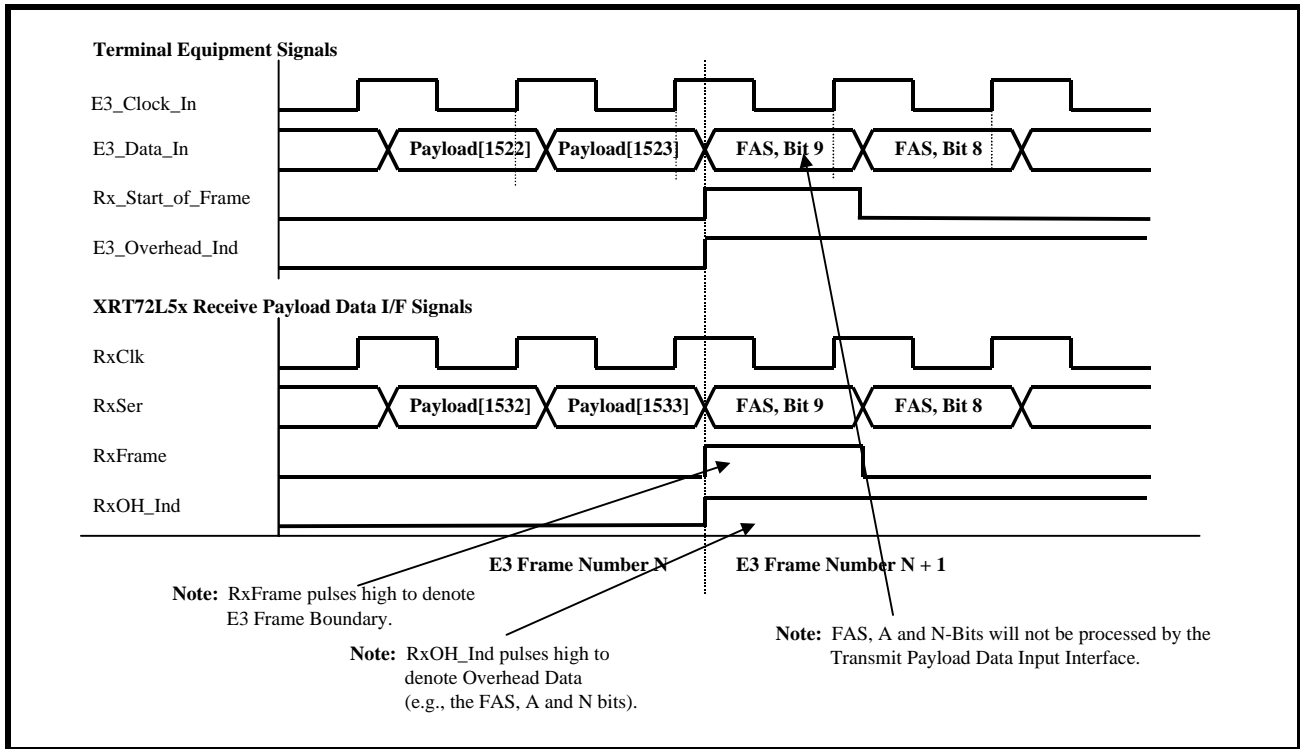
FIGURE 197. AN ILLUSTRATION OF THE BEHAVIOR OF THE SIGNALS BETWEEN THE RECEIVE PAYLOAD DATA OUTPUT INTERFACE BLOCK OF THE XRT72L52 AND THE TERMINAL EQUIPMENT
