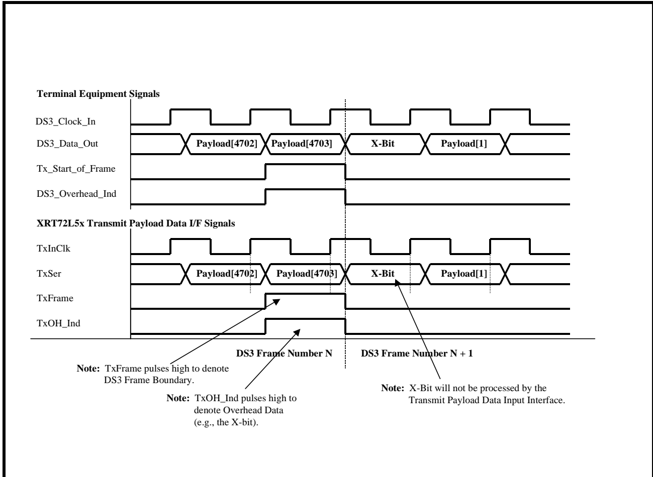
FIGURE 37. BEHAVIOR OF THE TERMINAL INTERFACE SIGNALS BETWEEN THE XRT72L52 AND THE TERMINAL EQUIPMENT (DS3 MODE 3 OPERATION)
