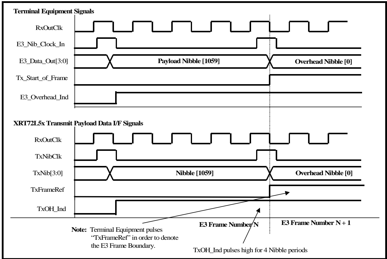
FIGURE 154. BEHAVIOR OF THE TERMINAL INTERFACE SIGNALS BETWEEN THE XRT72L52 AND THE TERMINAL EQUIPMENT (E3 MODE 5 OPERATION)
