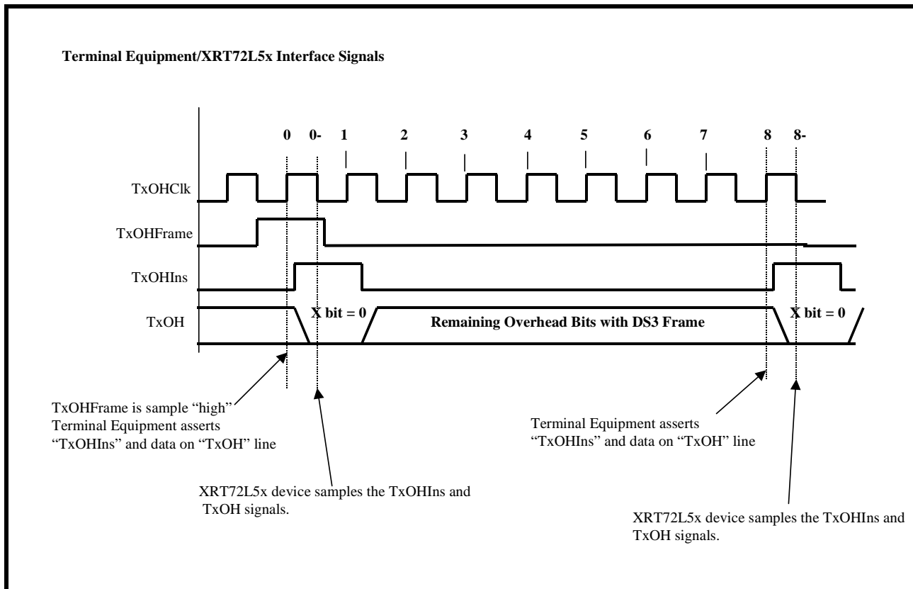
FIGURE 46. ILLUSTRATION OF THE SIGNAL THAT MUST OCCUR BETWEEN THE TERMINAL EQUIPMENT AND THE XRT72L52, IN ORDER TO CONFIGURE THE XRT72L52 TO TRANSMIT A YELLOW ALARM TO THE REMOTE TERMINAL EQUIPMENT
