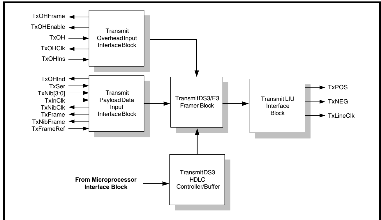
FIGURE 30. THE XRT72L52 TRANSMIT SECTION CONFIGURED TO OPERATE IN THE DS3 MODE
