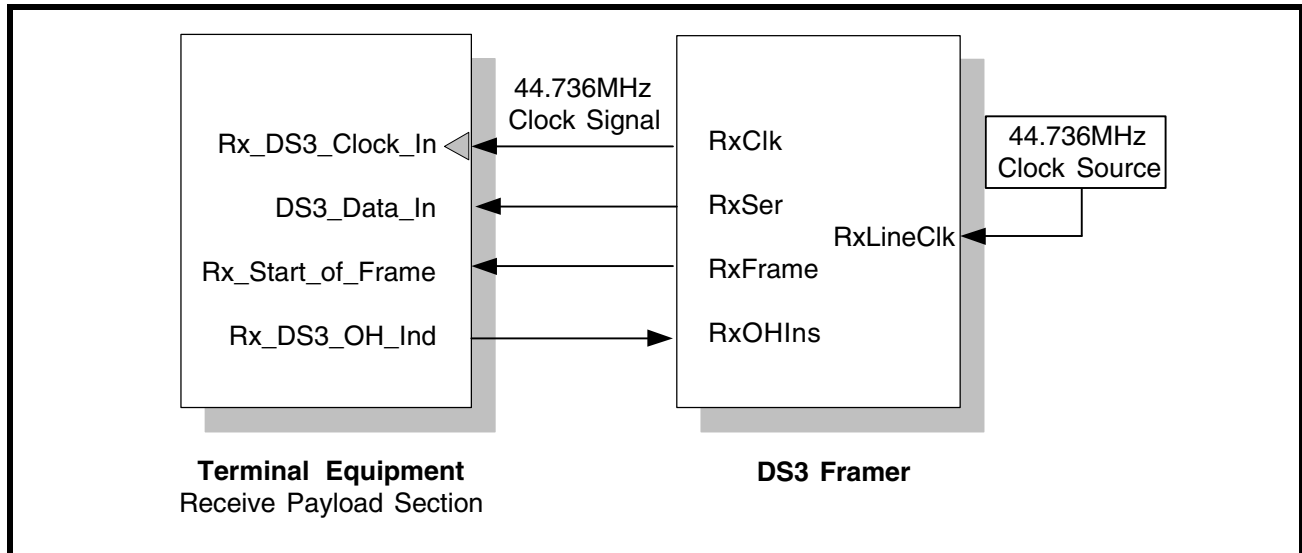
FIGURE 81. THE XRT72L52 DS3/E3 FRAMER IC BEING INTERFACED TO THE RECEIVE TERMINAL EQUIPMENT (SERIAL MODE OPERATION)
