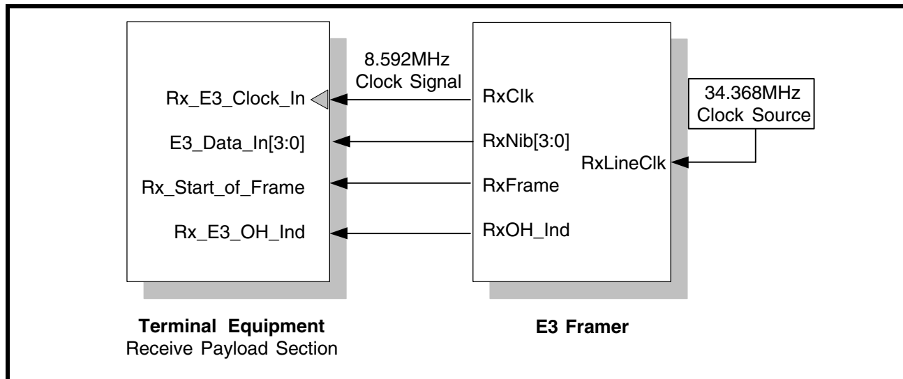
FIGURE 198. THE XRT72L52 DS3/E3 FRAMER IC BEING INTERFACED TO THE RECEIVE SECTION OF THE TERMINAL EQUIPMENT (NIBBLE-PARALLEL MODE OPERATION)
