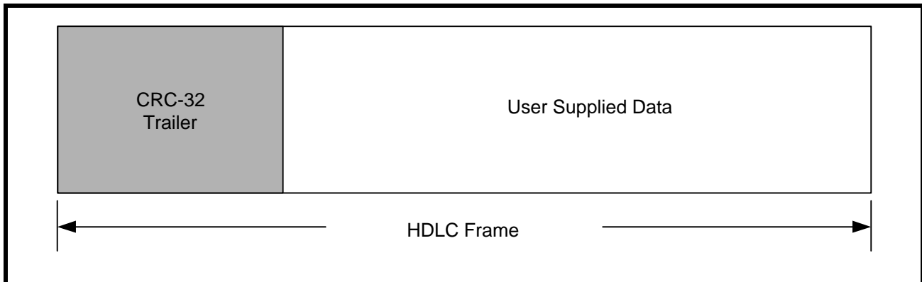
FIGURE 203. AN OUTBOUND HDLC FRAME WHEN CRC-32 IS SELECTED.
