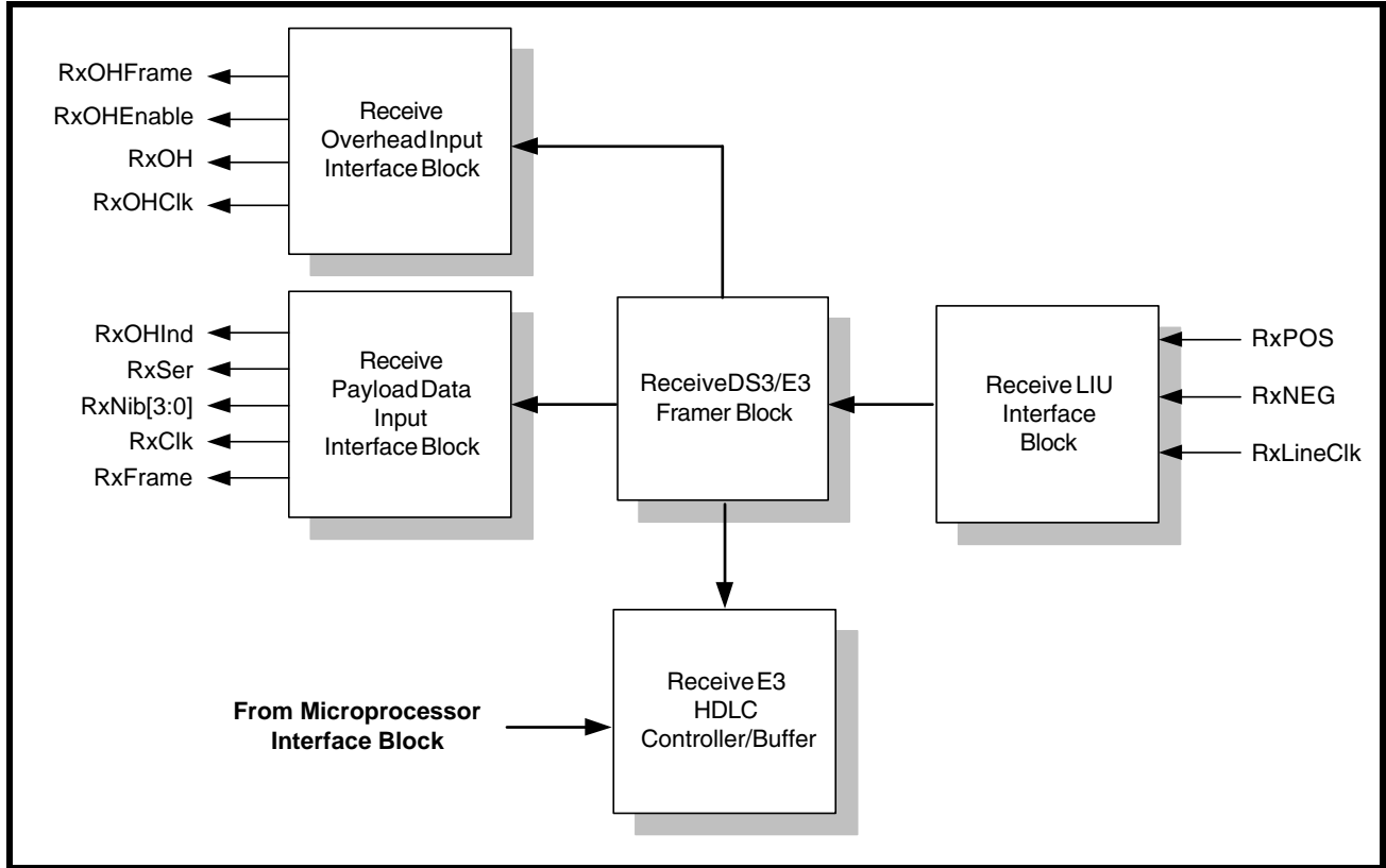
FIGURE 173. THE XRT72L52 RECEIVE SECTION CONFIGURED TO OPERATE IN THE E3 MODE
