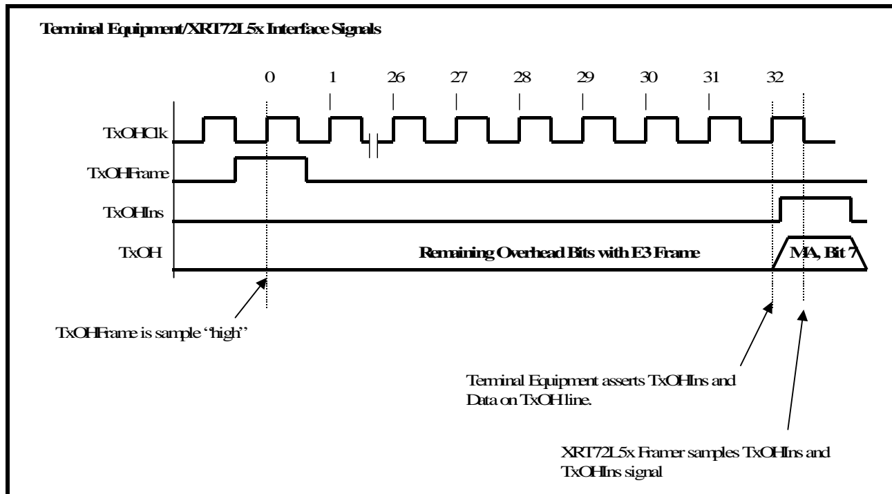
FIGURE 159. ILLUSTRATION OF THE SIGNAL THAT MUST OCCUR BETWEEN THE TERMINAL EQUIPMENT AND THE XRT72L52, IN ORDER TO CONFIGURE THE XRT72L52 TO TRANSMIT A YELLOW ALARM TO THE REMOTE TERMINAL EQUIPMENT
