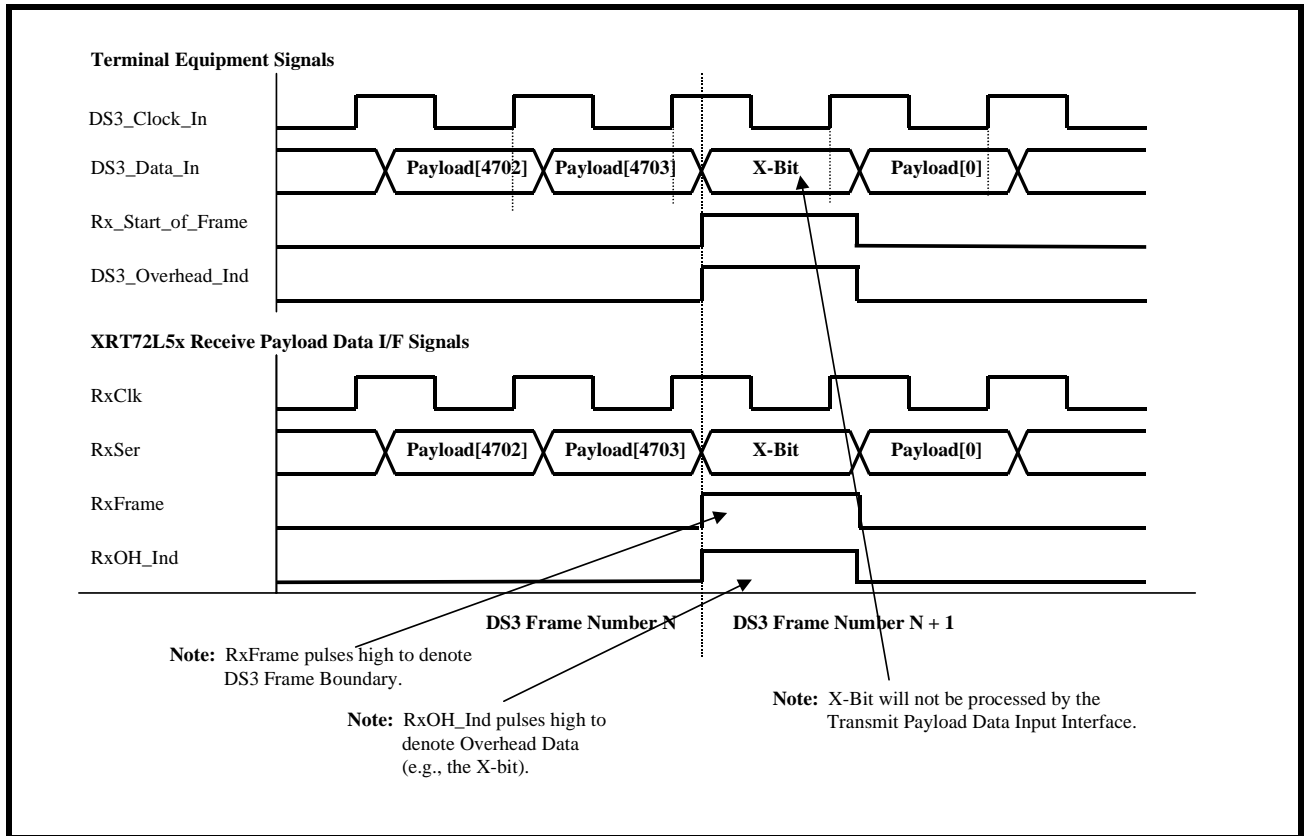
FIGURE 82. AN ILLUSTRATION OF THE BEHAVIOR OF THE SIGNALS BETWEEN THE RECEIVE PAYLOAD DATA OUTPUT INTERFACE BLOCK OF THE XRT72L52 AND THE TERMINAL EQUIPMENT (SERIAL MODE OPERATION)
