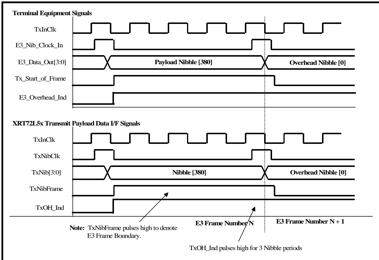
FIGURE 99. BEHAVIOR OF THE TERMINAL INTERFACE SIGNALS BETWEEN THE XRT72L52 AND THE TERMINAL EQUIPMENT (E3 MODE 6 OPERATION)
