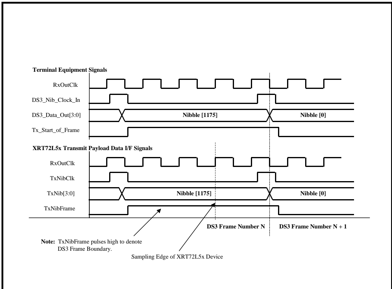
FIGURE 39. BEHAVIOR OF THE TERMINAL INTERFACE SIGNALS BETWEEN THE XRT72L52 AND THE TERMINAL EQUIPMENT (MODE 4 OPERATION)
