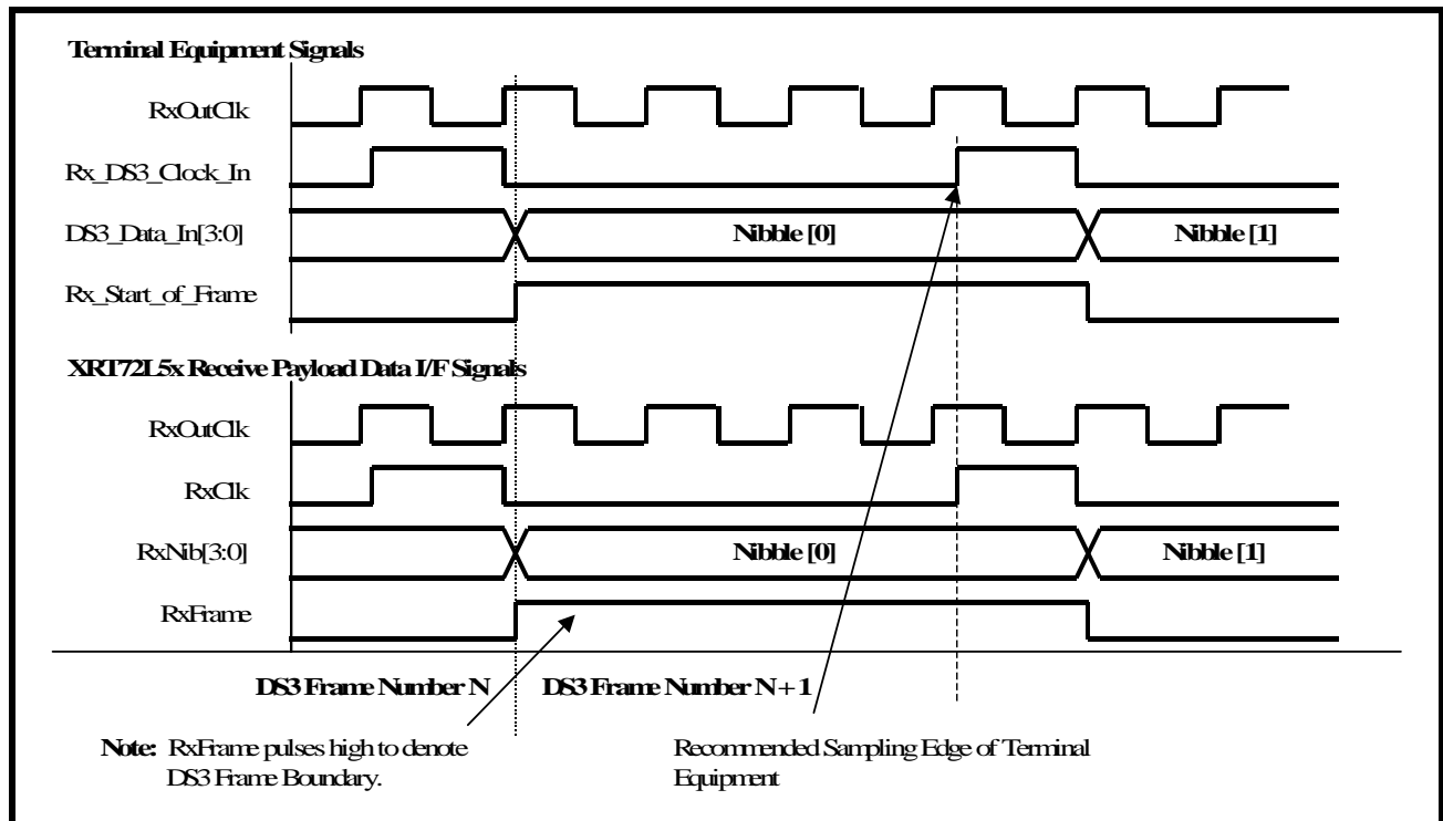
FIGURE 84. AN ILLUSTRATION OF THE BEHAVIOR OF THE SIGNALS BETWEEN THE RECEIVE PAYLOAD DATA OUTPUT INTERFACE BLOCK OF THE XRT72L52 AND THE TERMINAL EQUIPMENT (NIBBLE-MODE OPERATION).
