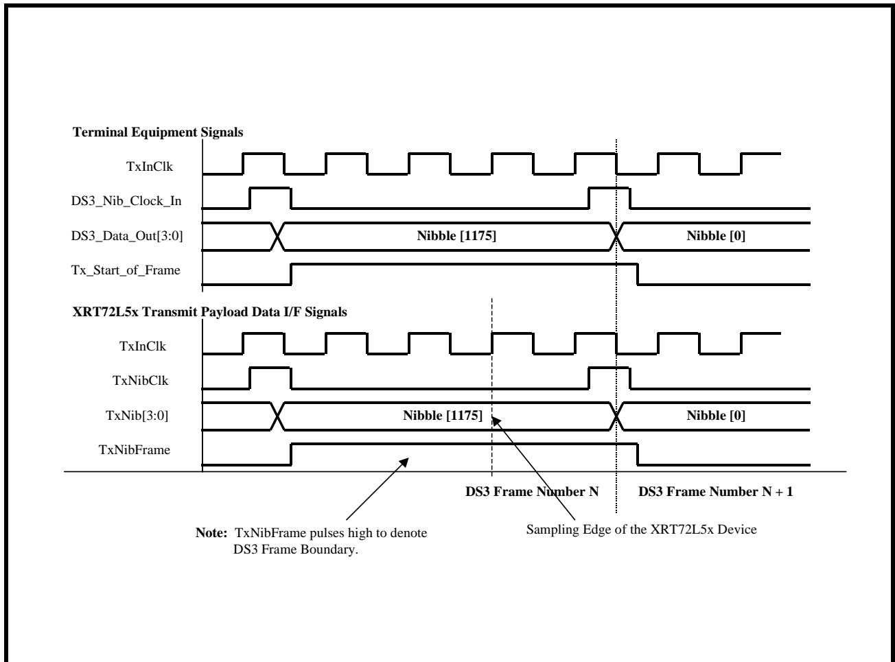
FIGURE 43. BEHAVIOR OF THE TERMINAL INTERFACE SIGNALS BETWEEN THE XRT72L52 AND THE TERMINAL EQUIPMENT (DS3 MODE 6 OPERATION)
