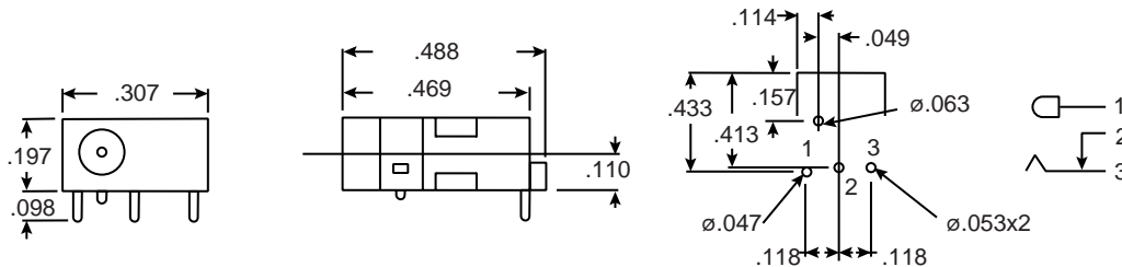
Dimensions (In.)
