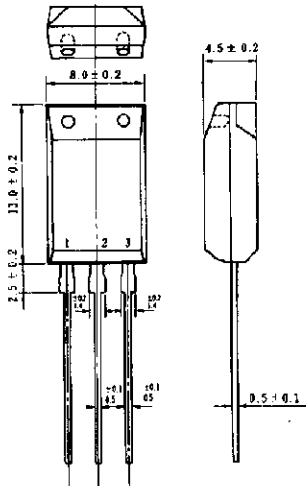
Electrode Connection 1. Base 2. Collector 3. Emitter
