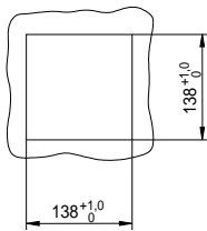
Panel cutout
