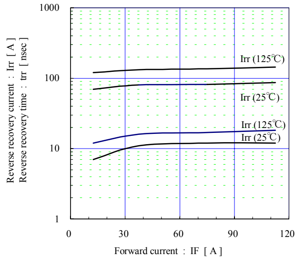
Reverse recovery characteristics (typ.) V_{cc}=300\text{V} , V_{GE}=\pm 15\text{V} , R_g=47\Omega
