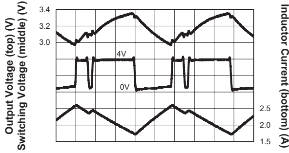
Time (250ns/div)
