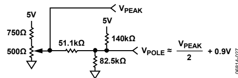
Figure 22. Deriving V_{POLE} from V_{PEAK} with Potentiometer for UTP Cable
