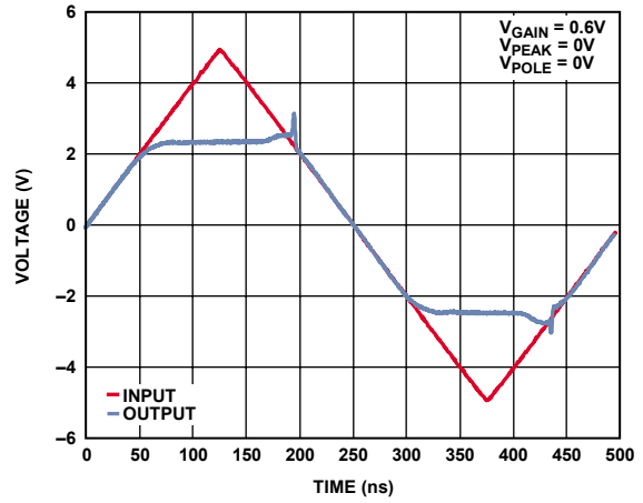
Figure 10. Overdrive Recovery
