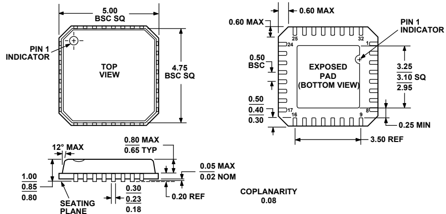
Figure 35. 32-Lead Lead Frame Chip Scale Package [LFCSP_VQ] 5 mm × 5 mm Body, Very Thin Quad (CP-32-2) Dimensions shown in millimeters
