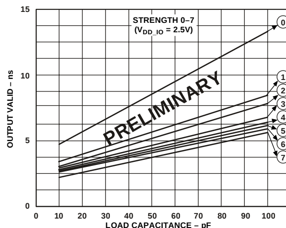
Figure 42. Typical Output Valid ( V_{DD\_IO} = 2.5 V ) vs. Load Capacitance at Max Case Temperature and Strength 0–7 1
