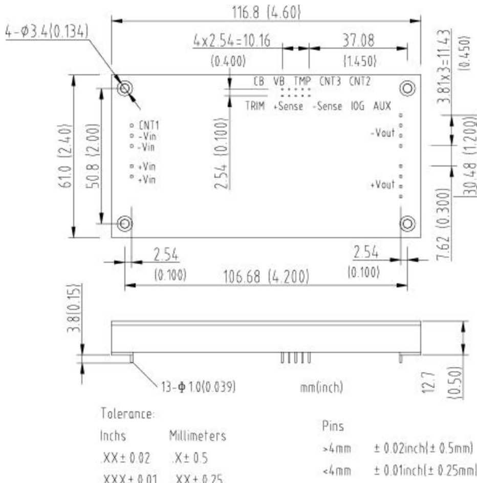
AIF25R48N-6 (pin side view)
