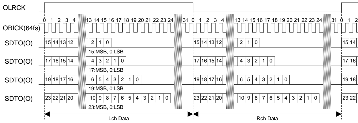
Figure 7. MSB Timing
