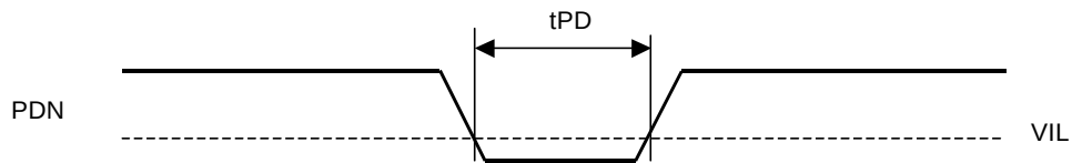
Figure 9. Power-down &amp; Reset Timing
