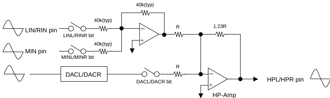
Figure 30. Summation circuit for headphone amp output
