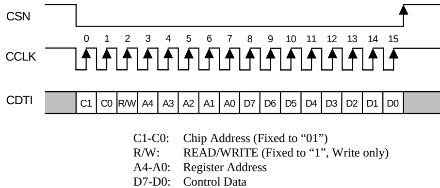
Figure 20. 3-wire Serial Control I/F Timing
