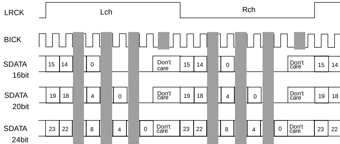
Figure 12. Mode 2 Timing
