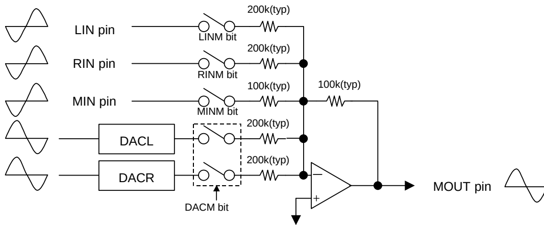
Figure 31. Summation circuit for MOUT
