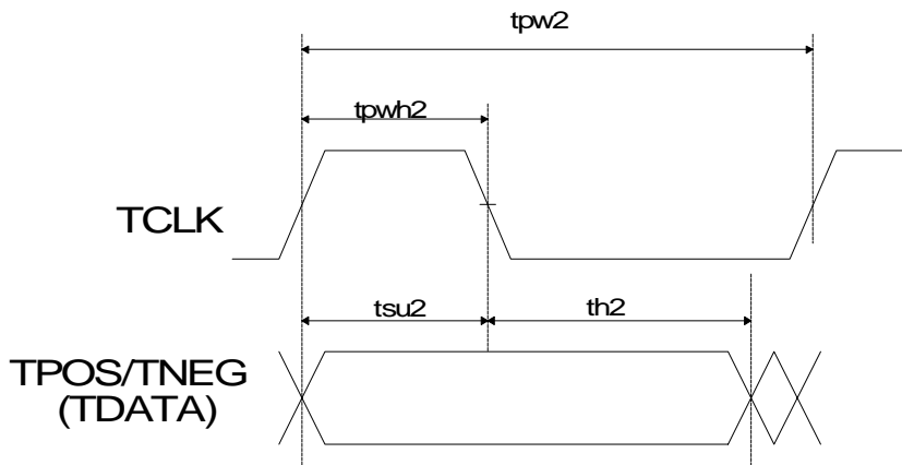
Figure 3. Transmit Clock and Data Switching Characteristics
