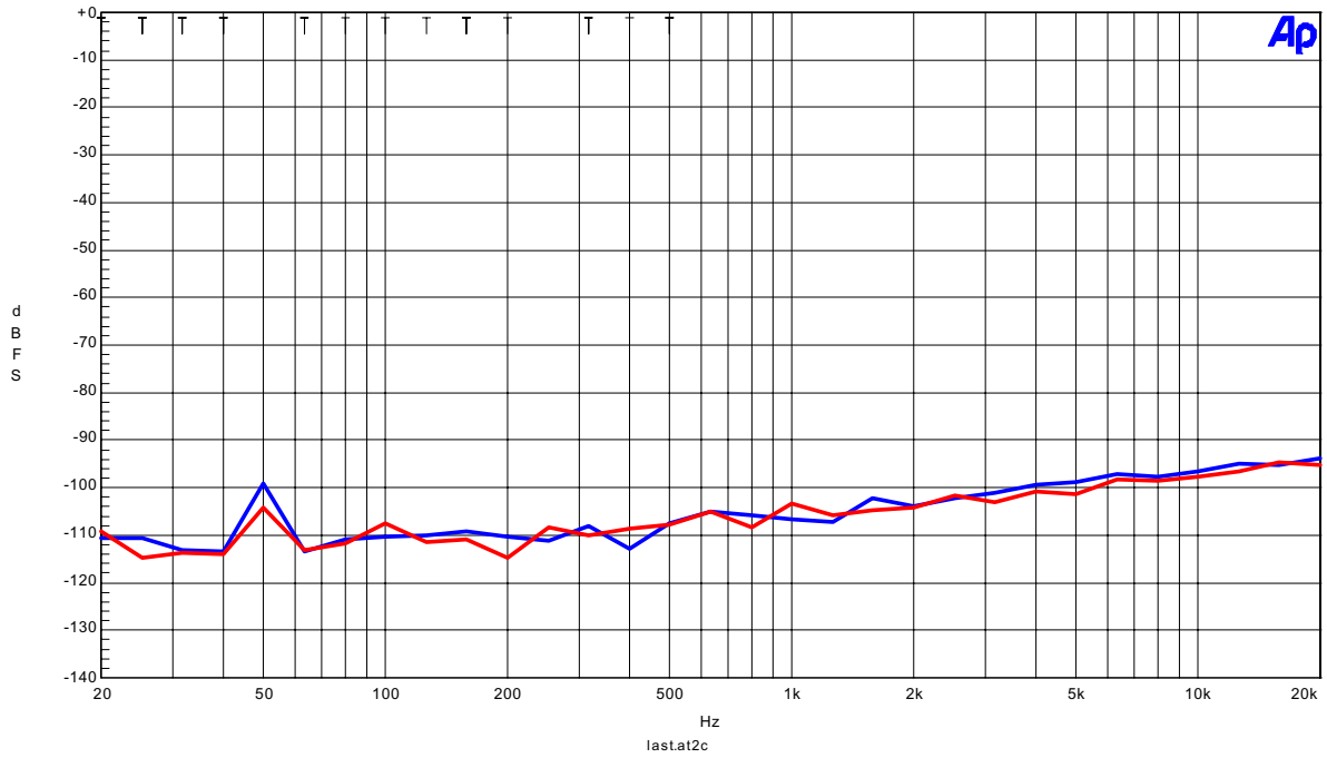
Figure 13. Crosstalk
