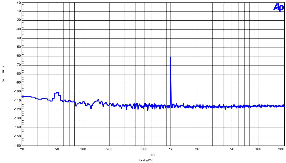
Figure 15. FFT Plot
