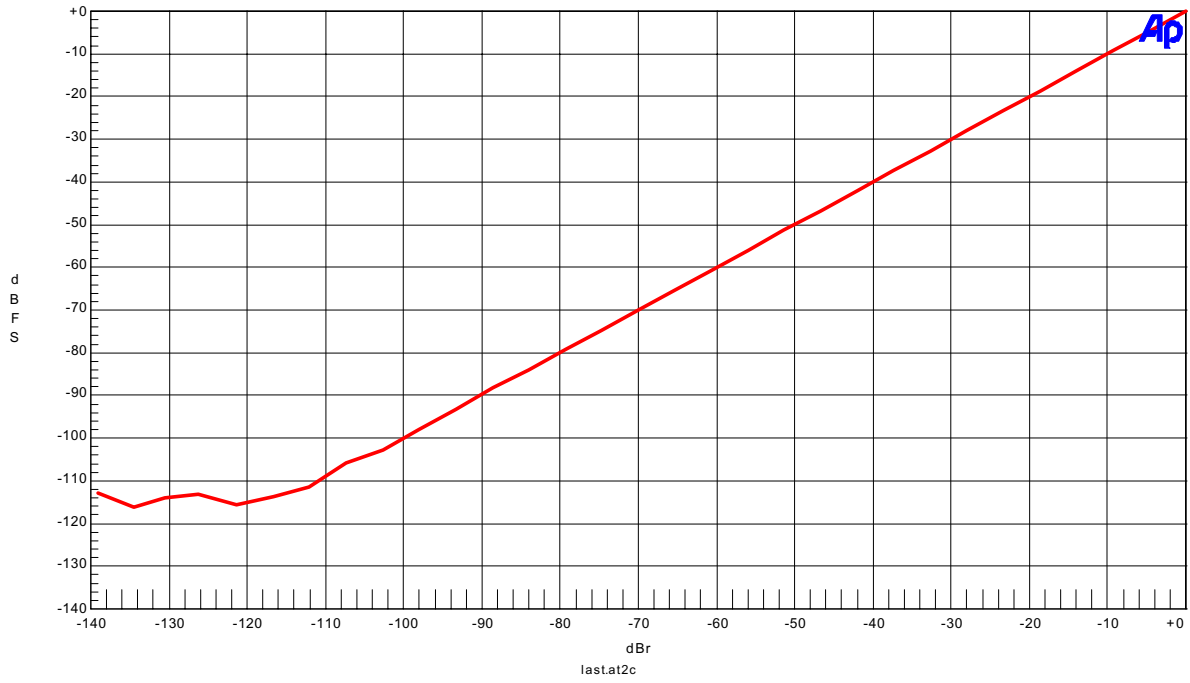
Figure 3. Linearity
