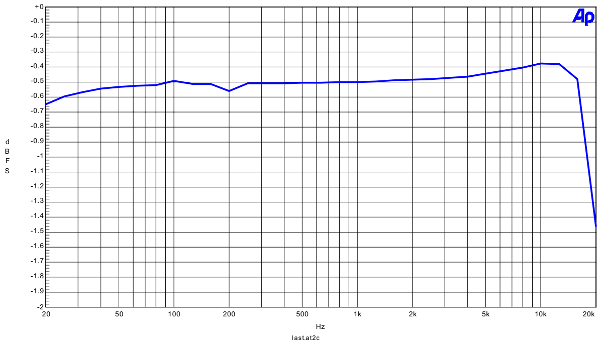
Figure 4. Frequency Response
