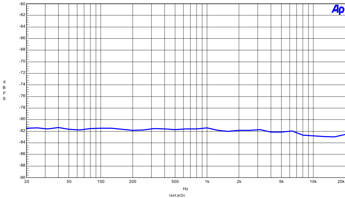
Figure 2. THD+N vs. Input Frequency
