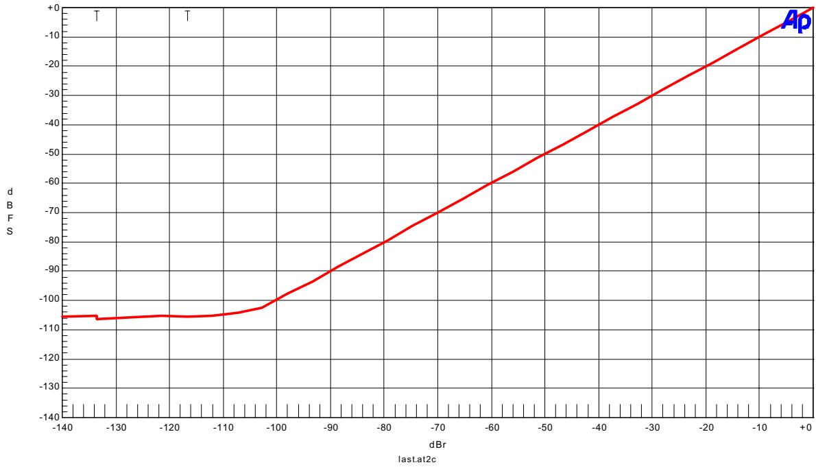
Figure 11. Linearity
