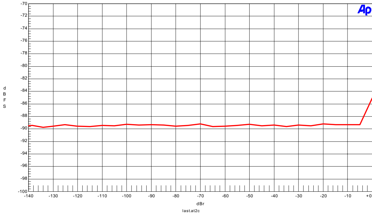
Figure 1. THD+N vs. Input Level
