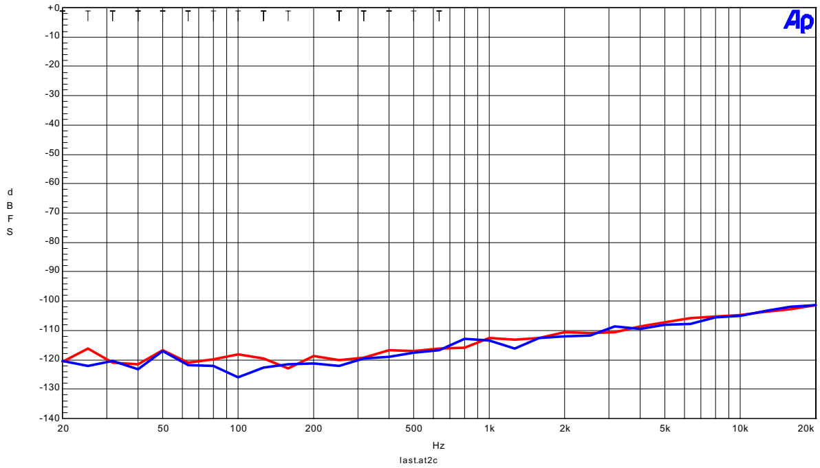
Figure 5. Crosstalk
