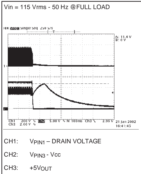
Figure 17. TURN-OFF
