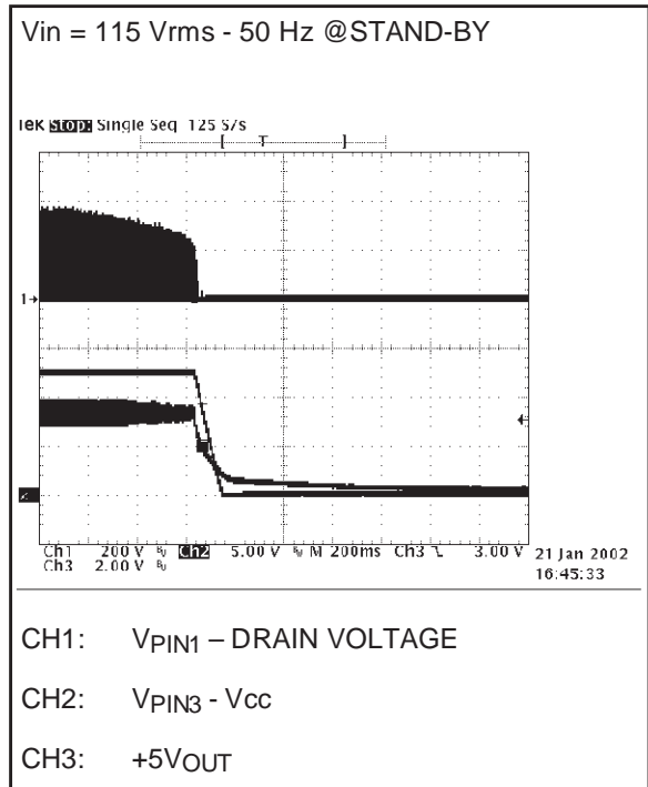
Figure 18. TURN-OFF
