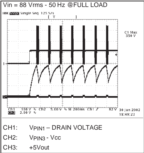
Figure 26. SWITCH ON WITH +5V SHORTED
