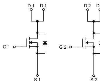
N-Channel MOSFET
